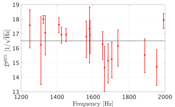
FIG. 6. Depth values corresponding to the 95% detection efficiency, \mathcal{D}^{95\%} , obtained for 18 0.1 Hz frequency bands between 1200 and 2000 Hz, along with their corresponding 2\sigma_F uncertainties in red markers. The average of the measured depths at different frequencies being \langle \mathcal{D}^{95\%} \rangle_{\text{High}} = 16.5 \text{ Hz}^{-1/2} .
