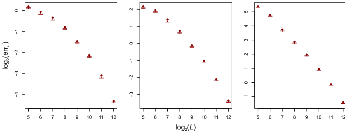
Figure 1: Plot of \log_2(\text{err}_L) against \log_2(L) for q = 500, 1000, 5000 going from left to right. The bars give the first and third quartiles of \log_2(\text{err}_L) over the 100 simulations, and the circles give maximum values.
