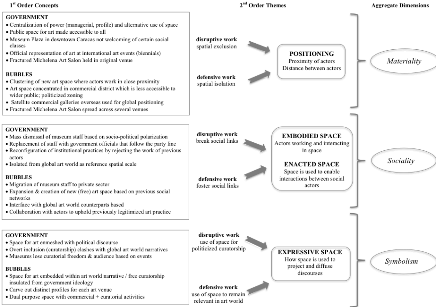
Figure 3. Data Structure
