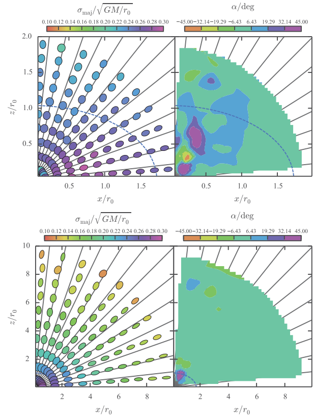
Figure 8. Tilt of the stellar halo for (b/a)_{\text{NFW}} = 0.9 , (c/a)_{\text{NFW}} = 0.8 model in the (x, z) plane: see Fig. 7 for details.
