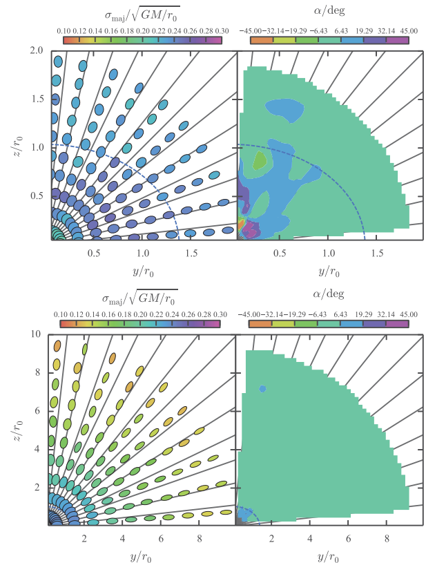
Figure 9. Tilt of the stellar halo for (b/a)_{\text{NFW}} = 0.9 , (c/a)_{\text{NFW}} = 0.8 model in the (y, z) plane: see Fig. 7 for details.
