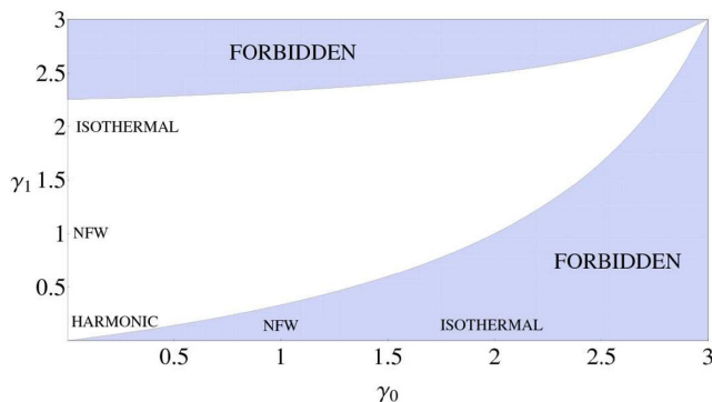
Figure 3. The domain of allowed cusp slope transformations. The final cusp slope \gamma_1 is plotted against the initial cusp slope \gamma_0 . Shaded regions cannot be reached by adiabatic changes. The upper line corresponds to \gamma_1(\gamma_0, -1) (the Keplerian limit) and the lower line to \gamma_1(\gamma_0, 2) (the harmonic limit).
