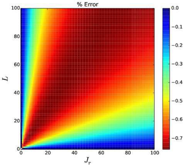
Figure 2. Distribution of percentage error with actions for the case \alpha = 1.5 . One can see a definite systematic trend that could be removed with an astute choice of first-order correction.
