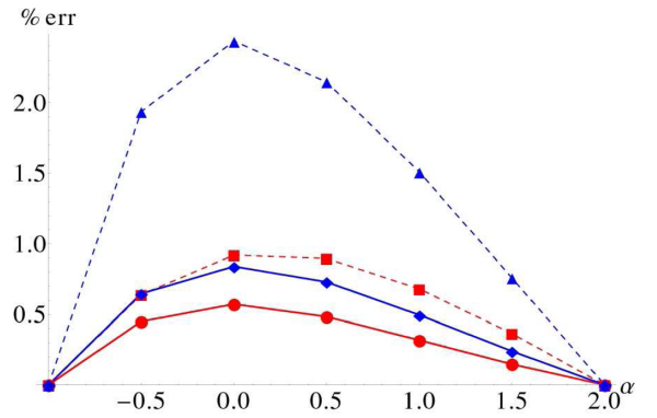
Figure 1. Absolute percentage errors against power-law index ( \alpha = 0 corresponds to the isothermal sphere). The dashed lines correspond to the original approximation, and the solid lines include first-order corrections. Blue lines are maximum absolute percentage errors across the action grid, red lines are the mean absolute percentage errors. One can see that the first-order corrections reduce the maximum error significantly, and also have a noticeable effect on the mean error.
