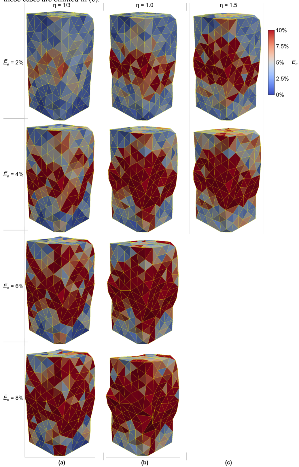
Figure 18: Discrete element predictions of the spatial distribution of the effective strain E_e (shown on the deformed configurations) in the idealised cermet specimen at three applied
