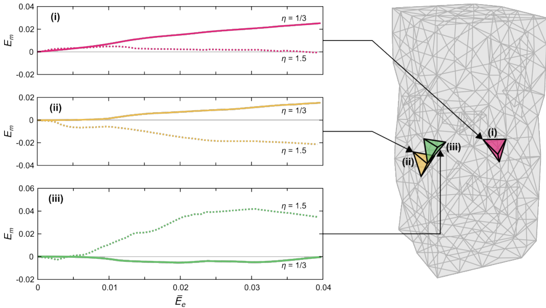
Figure 19: Discrete element predictions of the evolution of the mean strain E_m with the macroscopic strain \bar{E}_e in three selected tetrahedra within the assembly of spherical particles analysed here. The three tetrahedra are indicated in the specimen and the E_m - \bar{E}_e curves shown for \eta = 1/3 and \eta = 1.5 .
