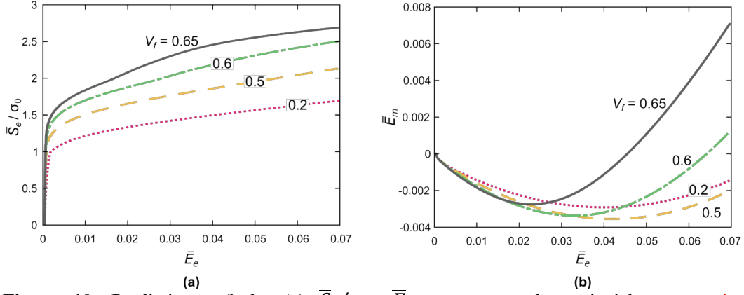
Figure 10: Predictions of the (a) \bar{S}_e/\sigma_0 - \bar{E}_e response under uniaxial compression ( \eta = 1/3 ) and (b) corresponding strain paths in \bar{E}_m - \bar{E}_e space for the FCC unit cell with particle volume fractions in the range 0.2 \leq V_f \leq 0.65 and initial matrix porosity f_0 = 0.1 .
