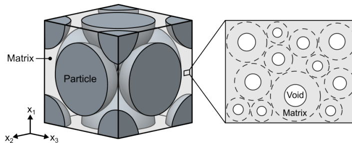
Figure 9: Sketch of the 3D periodic unit cell comprising nearly rigid spherical particles in a face-centred-cubic arrangement with the interstitial spaces filled with a porous plastic matrix.
