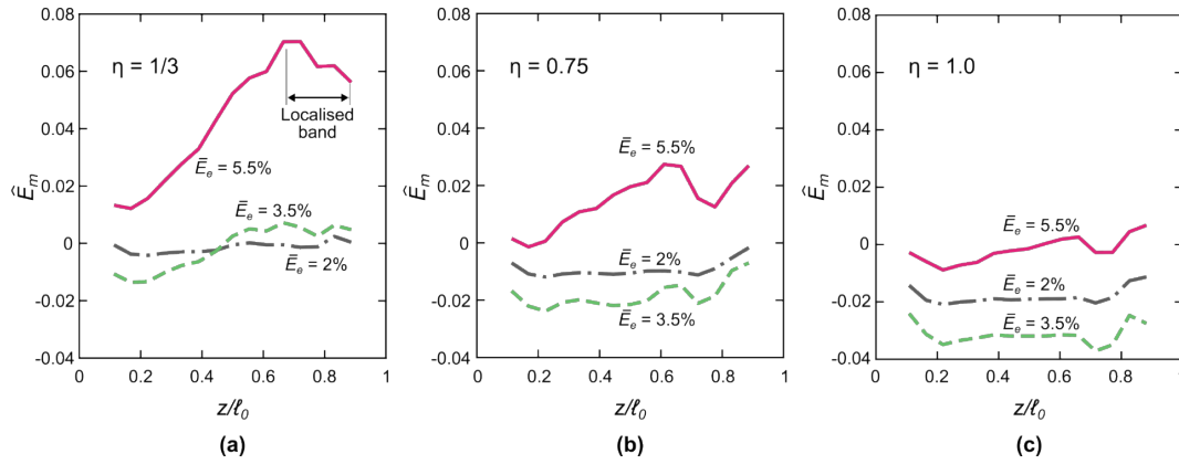
Figure 8: Digital volume correlation (DVC) measurements of the average volumetric strain \hat{E}_m as a function of the normalised axial co-ordinate z/\ell_0 . Measurements are shown for the specimens deformed under stress paths (a) \eta = 1/3 , (b) \eta = 0.75 and (c) \eta = 1.0 for overall strain levels \bar{E}_e = 0.02, 0.035 and 0.055 in each case.
