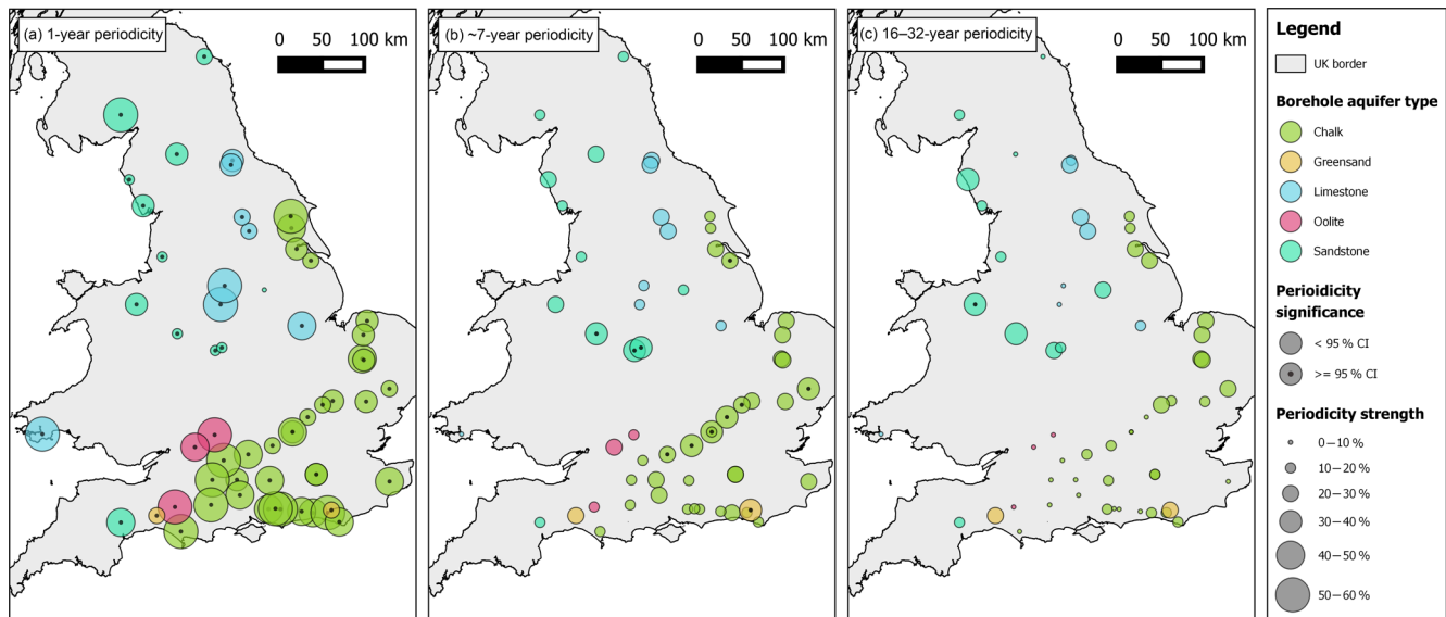
Figure 6. Maps showing strength (percentage of the original time series standard deviation) and significance of the (a) 1-year, (b) \sim 7-year, and (c) 16–32-year periodicity bands. No periodicity strength was found to be above 60 % of the original signal.
