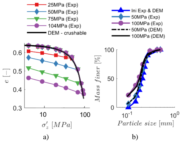
Figure 1. DEM and experimental curves of a) oedometric compression test and b) PSD evolution.
