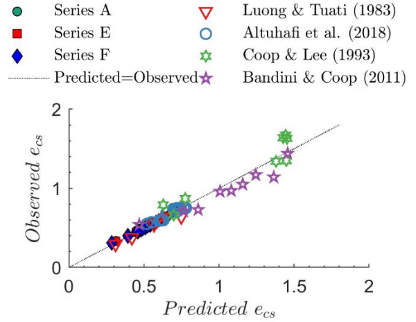
Figure 7. Critical state values for evolving grading: predicted values from the CSP plotted against observed values.
