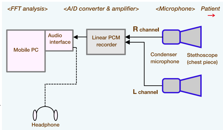
Fig. 2. Block diagram. A/D, analog-to-digital; FFT, fast Fourier transform; PC, personal computer; PCM, pulse code modulation.
