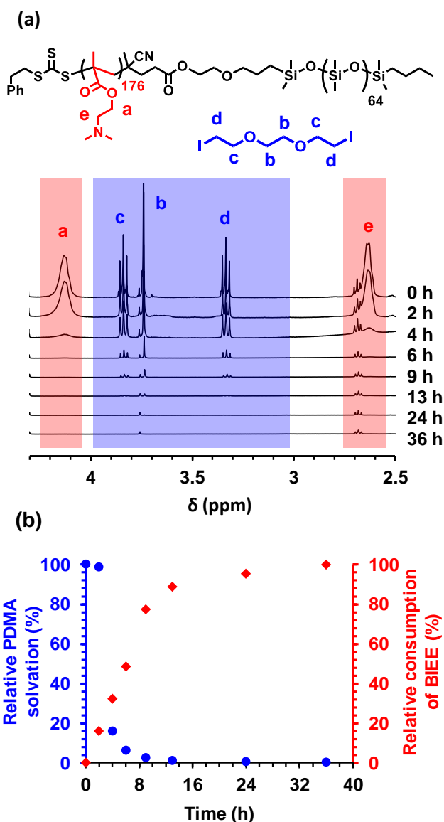
Figure 10. (a) 1 H NMR spectra recorded after various intervals at 20 °C for the cross-linking of PDMS 66 -PDMA 176 vesicles using BIEE at a BIEE/DMA molar ratio of 0.15. This quaternization reaction was performed at 25% w/w in D5 silicone oil and dispersions were diluted to 2.5% w/w in chloroform for 1 H NMR analysis. The gradual disappearance of signals a and e assigned to the PDMA block at 4.15 ppm and 2.65 ppm respectively, and also the BIEE signals at 3.3-3.9 ppm indicates the onset of cross-linking. (b) Kinetics of BIEE cross-linking PDMS 66 -PDMA 176 vesicles. The degree of solvation of the PDMA block was determined using its oxymethylene signal a at 4.15 ppm. The extent of BIEE consumption was monitored using signals b , c and d . All signals were normalized relative to a suitable external standard (0.1 M pyridine in toluene- d 8 ) contained within a coaxial inner tube.
