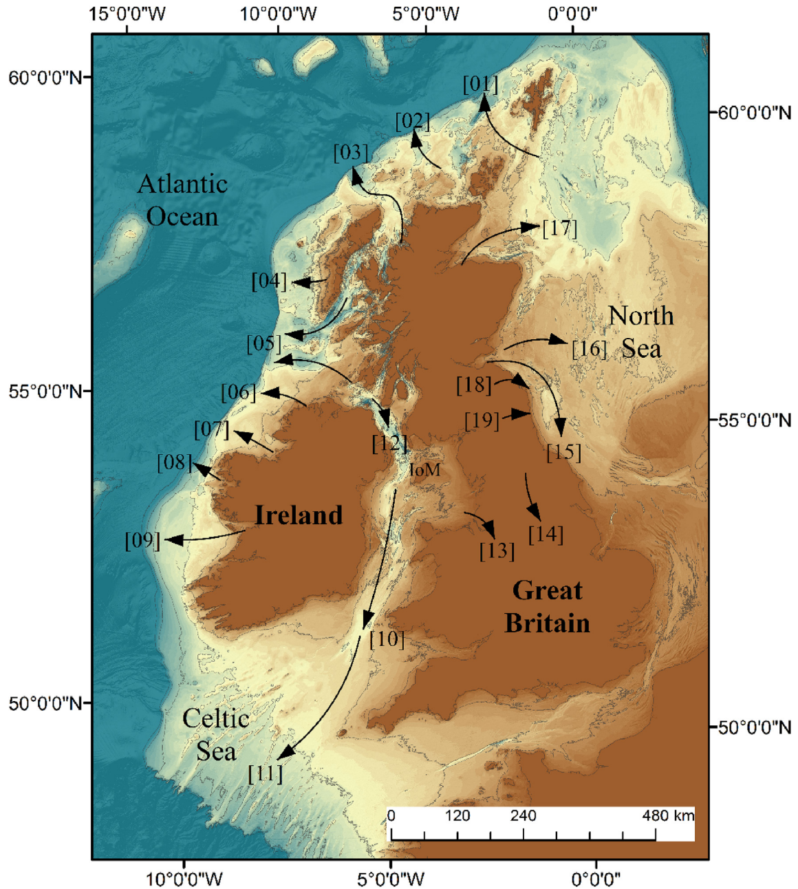
Fig. 1. The location of BISS palaeo ice streams. IoM = Isle of Man. Grey contours show contemporary bathymetry from -240 m in 40 m intervals.
