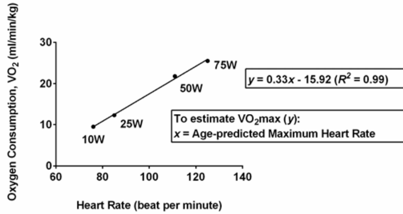
Figure 1a: An Example of Linear Regression for Estimation of Maximal Oxygen Consumption ( VO_2\text{max} )
