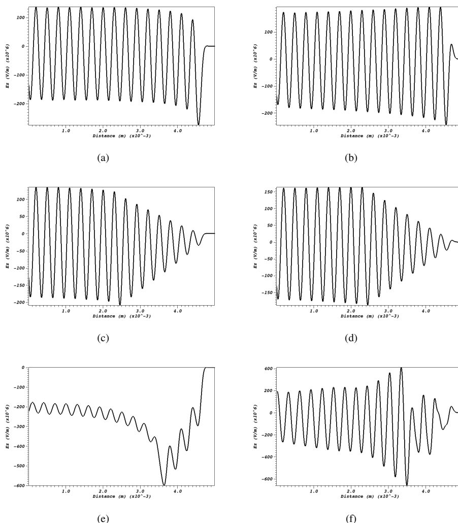
Figure 2: a,b) Single bunch of 8 nC, c,d) eight bunches with 1 nC each and separated by \lambda_p , e,f) eight bunches with 1 nC each and separated by \lambda_p/2 at the first time step and after 100 mm propagation into the plasma, respectively.
