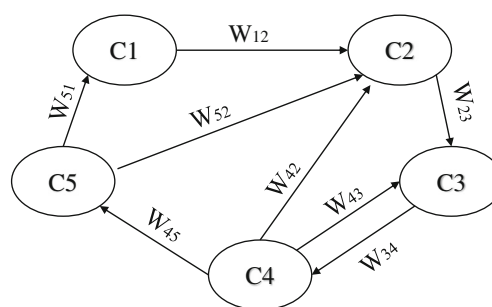
Fig. 1 A simple representation of an FCM, where C represents a concept and W denotes the interrelation between each pair of concepts (Navas de Maya et al. 2018)
