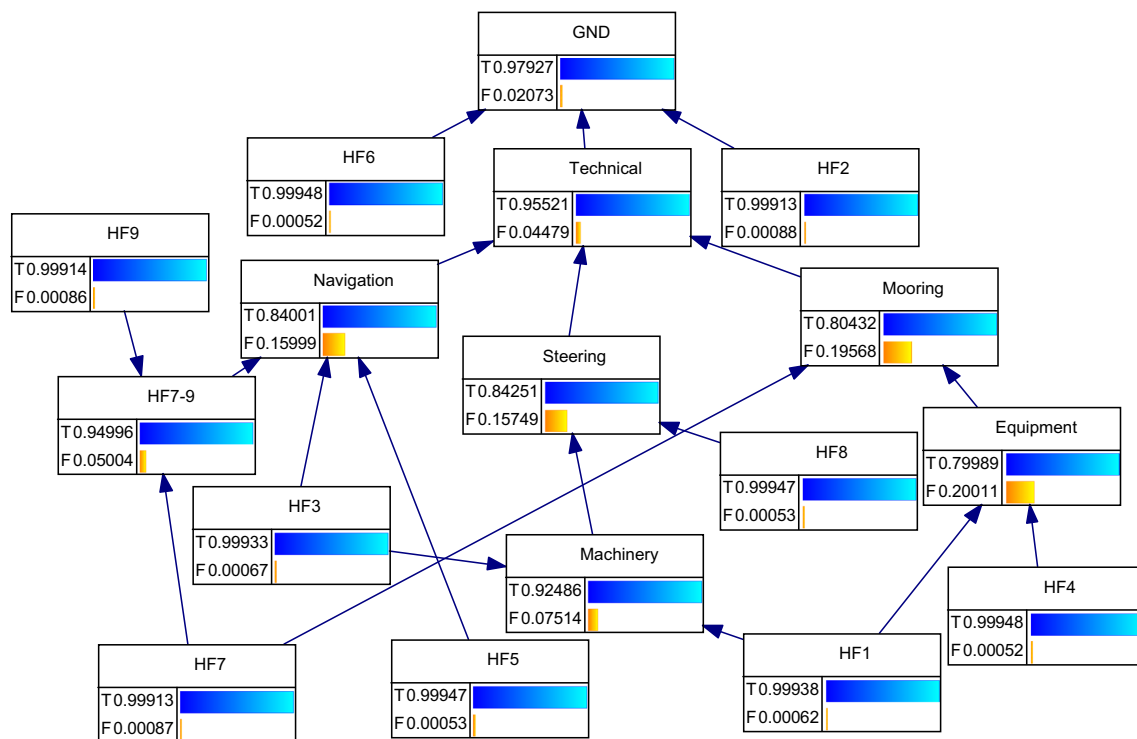
Fig. 3 BN model for the wreckage/stranding accident
