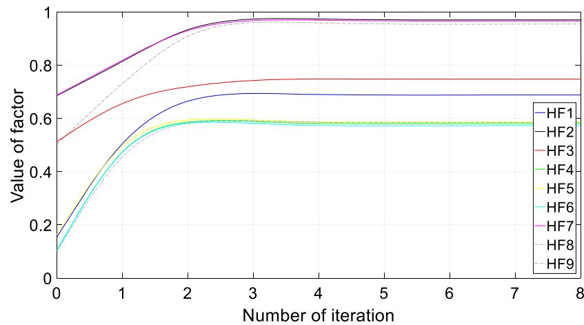
Fig. 2 Values of MALFCM for grounding/stranding accidents in general cargo vessels until equilibrium is reach. Period 2011–2016
