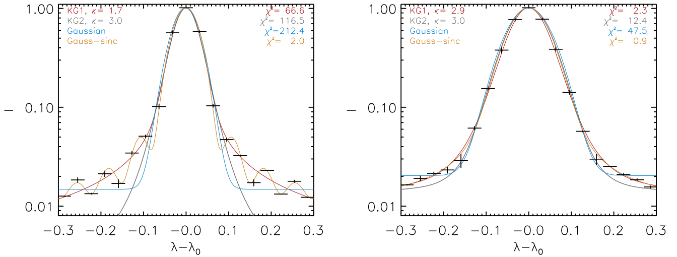
Figure 12. Modeled convolved Gaussian– \text{sinc}^2\lambda line profile using the EIS spectral pixel resolution of 0.022 \text{ \AA} for Fe XVI (left) and Fe XXIII (right). The Gaussian part of the profile in the left column represents Fe XVI and the right column Fe XXIII, and each has a noise level of 5%. Each line is fitted with (1) KG1 (pink), (2) KG2 (dark gray), (3) Gaussian (blue), and (4) Gaussian– \text{sinc}^2\lambda (orange). The reduced \chi^2 values for each fit are also shown.
