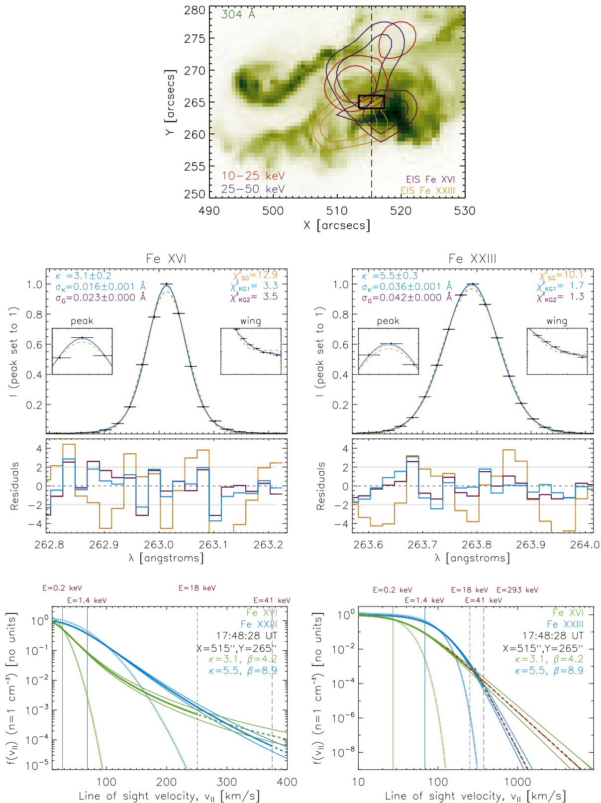
Figure 9. Top: SDO AIA 304 Å image of SOL2014-03-29T17:44 showing RHESSI and EIS contours (see legend) and one region (at t_3 : 17:48:28 UT) centered at [X ~ 515", Y ~ 265"], where line profiles of Fe XXIII and Fe XVI can be fitted by KG1 using the five criteria of Section 2. Middle row: both lines are fitted with a kappa-Gaussian, and they have different values of the \kappa index. The residuals and \chi^2 values show that the kappa-Gaussian fits are a better model than the single Gaussian fit. Bottom row: the kappa line profiles are converted to 1D velocity distributions f(v_{||}) using Equation (2) (and divided by the maximum value of f(v_{||}) ). The bottom left panel displays f(v_{||}) over the range of velocities fitted during the observation while the bottom right panel shows f(v_{||}) plotted over a larger range of v_{||} . At large v_{||} , a linear fit to \log f(v_{||}) vs. \log v_{||} (red lines) gives the velocity power index \beta , with values displayed in the legend.
