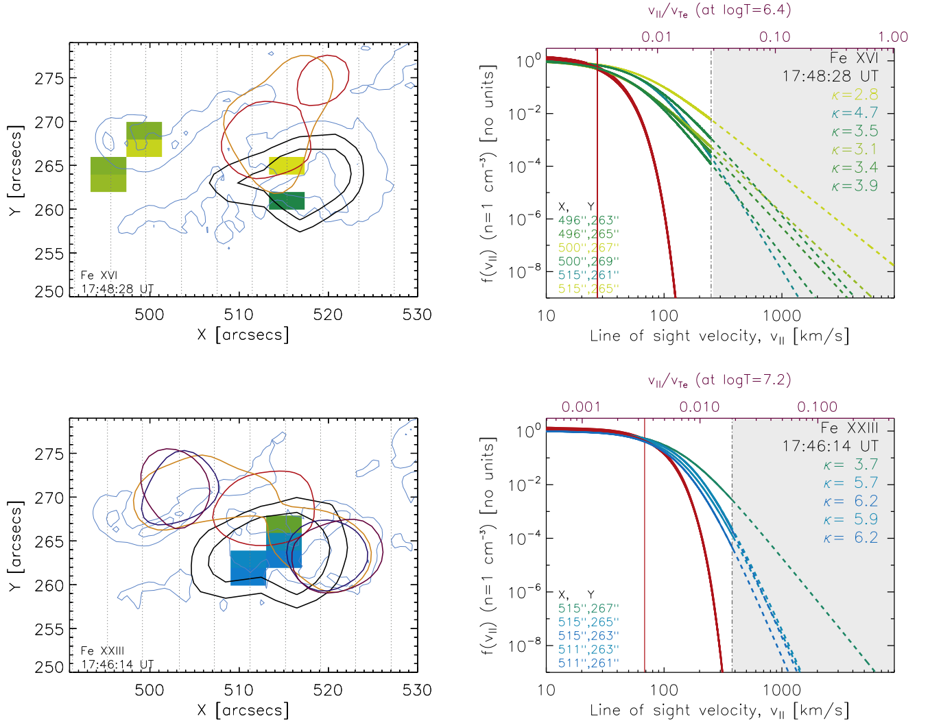
Figure 8. Left: Fe XVI (top) and Fe XXIII (bottom) index maps (re-plotted from Figure 7) at two different times (see maps). Right: for each region in the map (left), the forms of the possible ion velocity distributions are determined using Equation (2) and the observed fit values of \kappa index and \sigma_\kappa (corresponding colours). We are only interested in the form of f(v_{||}) , not the actual values ( n is set to 1 and f(v_{||}) is also divided by the maximum value for plotting). The red curve denotes the expected Maxwellian velocity distribution with the red vertical line denoting the ion thermal speed. For Fe XXIII, the distribution tends more toward a Maxwellian as the regions move away from the X-ray source (red contour) and toward the center of the Fe XXIII source (black contours). The gray dashed curve indicates the fit cut-off velocity. The errors for f(v_{||}) are not shown for clarity (see Figure 9). Error values for \kappa and W are shown in Table 1. v_{Te} = electron thermal speed at either \log T = 6.4 or \log T = 7.2 .
