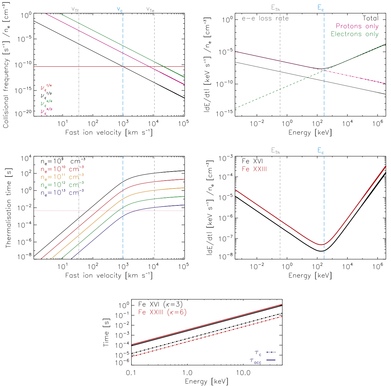
Figure 10. Top left: Fe XVI ( f ) collisional frequency in an electron ( e )–proton ( p ) background plasma for f – e interactions (red) and f – p interactions (black), vs. ion velocity ( km s^{-1} ). Top right: energy loss rate dE/dt vs. total ion kinetic energy (not energy per nucleon) for Fe XVI f – e and Fe XVI f – p collisions. The black curve is a combination of both interactions while the f – e (green) and f – p (pink) curves are also shown individually. The energy loss rates for e – e (gray) are also shown for comparison (note these are divided by n_e ). At the observed energies of interest, f – p collisions are the dominant interaction. Middle left: the thermalization times for the Fe XVI ions, due to different background electron number densities (where n_e = n_p ). Middle right: comparison of f – e and f – p energy loss rates for Fe XVI and Fe XXIII. The energy loss rate for Fe XXIII is 2\times larger than that for Fe XVI, which might account for the different \kappa indices observed for both ions. Bottom panel: comparison of the collisional (dashed) and acceleration (solid) times for Fe XVI (black) and Fe XXIII (red) using a number density of 10^{10} cm^{-3} .
