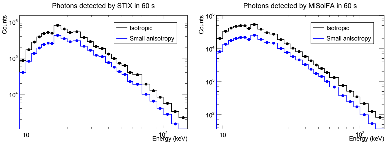
Fig. 9. Simulated measurements by STIX and MiSolFA within 1 min, with \cos \theta_S = 0.7-0.8 and \cos \theta_M = 0.9-1.0 .
