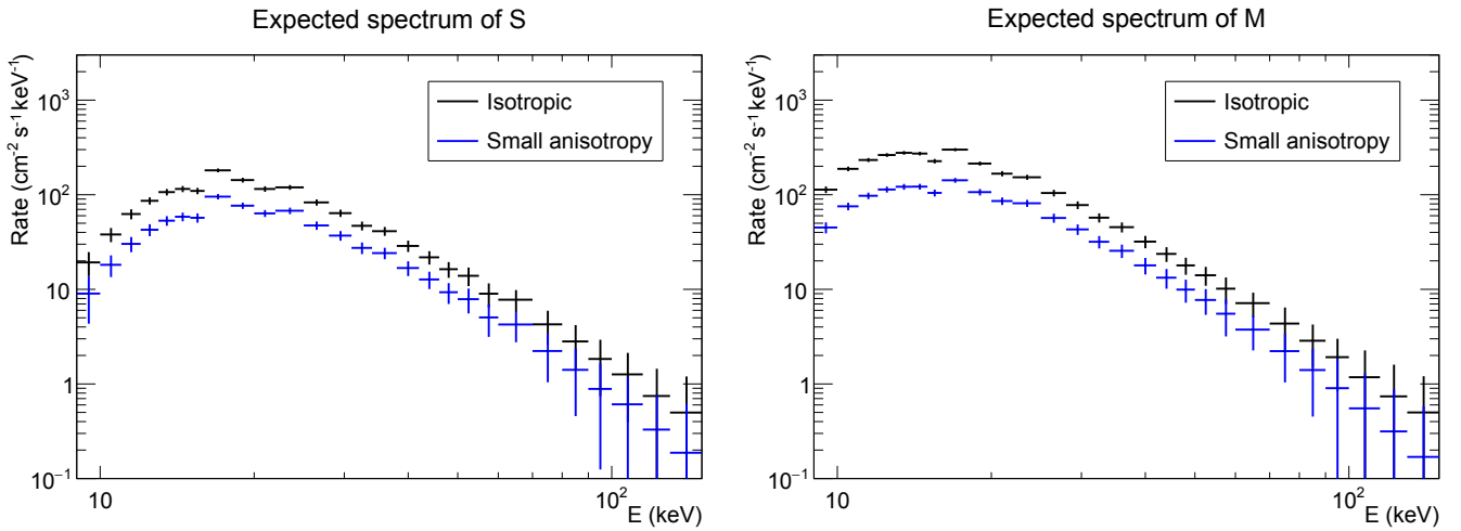
Fig. 8. Expected energy spectra with \cos \theta_S = 0.7-0.8 for STIX and \cos \theta_M = 0.9-1.0 for MiSolFA.
