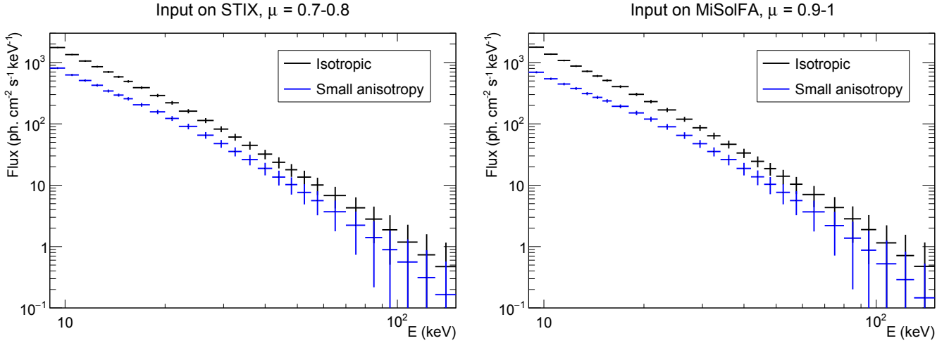
Fig. 7. Simulated input spectra with \cos \theta_S = 0.7-0.8 for STIX and \cos \theta_M = 0.9-1.0 for MiSolFA.
