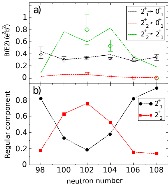
Fig. 18. (Color online) a) Comparison of the experimental reduced transition probabilities (open symbols) and the IBM-CM results (dashed lines) involving the 2_1^+ and 2_2^+ states. Experimental values are taken from Table 8 and from Ref. [58] for ^{178}\text{Hg} and Ref. [59] for ^{180}\text{Hg} b) IBM-CM results for the regular content (part of the wave function without particle-hole excitations) of the 2_1^+ and 2_2^+ states.
