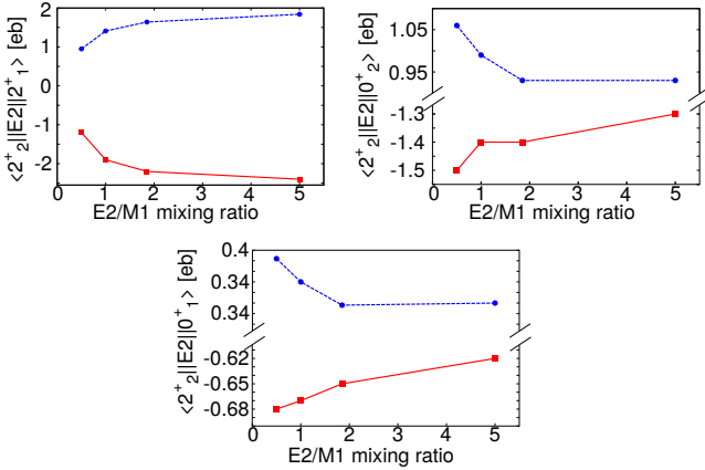
Fig. 14. (Color online) E2 and M1 matrix elements related to the 2_2^+ state in ^{182}\text{Hg} (red solid line) and ^{184}\text{Hg} (blue dashed line) resulting from the Coulomb-excitation data analysis performed assuming different values of the E2/M1 mixing ratio for the 2_2^+ \rightarrow 2_1^+ \gamma -ray transition.
