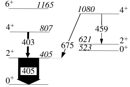
Fig. 10. Low-energy part of the level scheme of ^{186}\text{Hg} , relevant to the Coulomb-excitation analysis. Level and \gamma -ray transition energies are given in keV. Widths of the arrows are proportional to the measured \gamma -ray yields. Figure adapted from Ref. [20].
