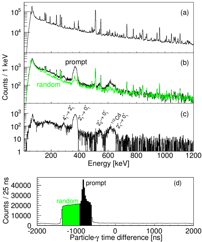
Fig. 1. (Color online) Gamma-ray spectra from the ^{184}\text{Hg} - ^{112}\text{Cd} experiment illustrating the data processing: (a) In-beam, un-conditioned \gamma -ray spectrum detected in the Miniball array during the EBIS pulse; (b) Gamma-ray spectrum collected in a prompt (black) and random (green) coincidence with detected ejectile / recoil particle(s) in the DSSSD; (c) Random-subtracted prompt \gamma -ray spectrum of ^{184}\text{Hg} . No Doppler-correction has been applied; (d) time difference between the detected \gamma ray and scattered particle with indicated prompt (black) and random (green) coincidence windows.
