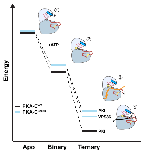
Fig. 6. Schematic of the energy landscape for PKA-C WT and PKA-C L205R , combining thermodynamics and MD simulations data. Relative free energy for the binding of ATP \gamma N, PKI, and VPS36 to PKA-C WT and PKA-C L205R derived from ITC data. (1) Apo PKA-C L205R samples mostly uncommitted states, with the Gly-rich loop partially occluded and the \alpha C helix turned outward. (2) Binary PKA-C L205R features a wired allosteric network for substrate binding, i.e., committed state. (3) Ternary PKA-C L205R complex with lower affinity for PKI (i.e., higher free energy relative to PKA-C WT ). The conformation of the activation loop of PKA-C L205R is in equilibrium between an unflipped and a sparsely populated flipped conformation. (4) PKA-C L205R /ATP \gamma N/VPS36 ternary complex features a flipped conformation of the activation loop with the electrostatic interactions between E86 and R194.
