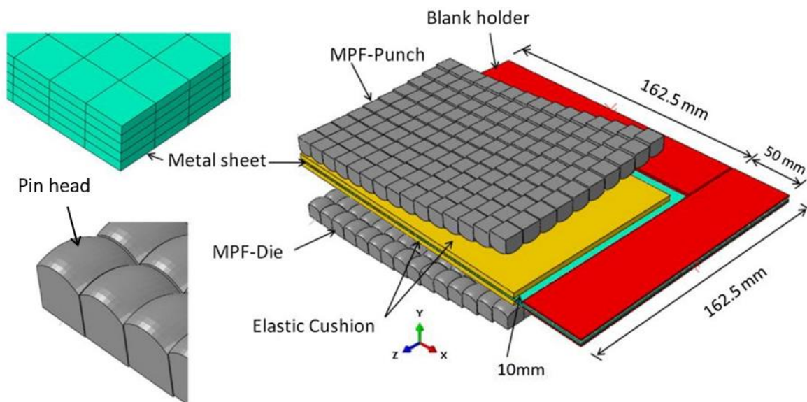
Figure 1. Schematic diagram of a MPF tool 4
