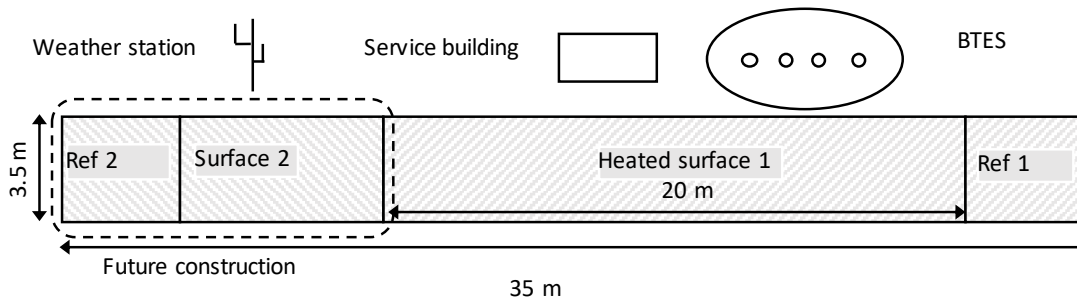
Figure 3.1: Main components and layout of the field station in Östersund.
