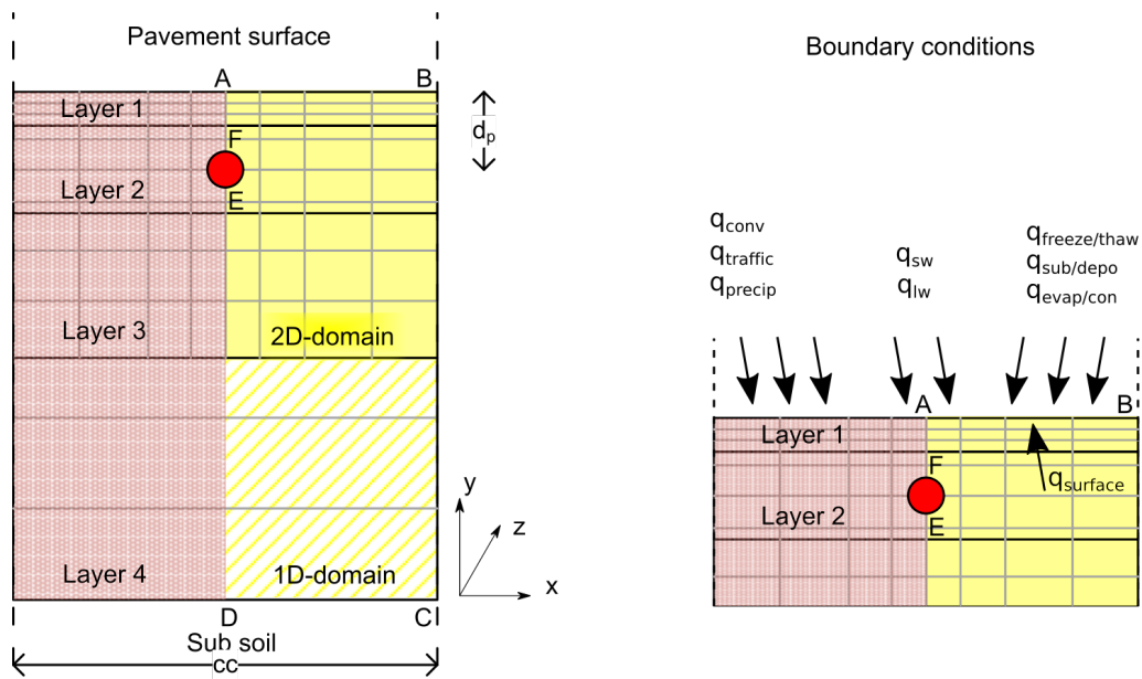
Figure 2.5: Left: Section plane representing segment, Seg_k , and the domain studied using FDM. The domain is divided into 1D and 2D regions. Right: Boundary conditions affecting the pavement surface.
