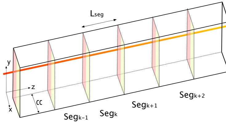
Figure 2.4: Geometrical model of 3D domain with segments used for the fluid temperature calculations.
