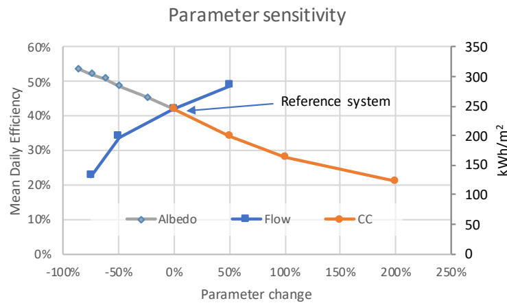
Figure 2.9: Calculated mean value of the daily efficiency for different variations of fluid flow, albedo, and pipe spacing.
