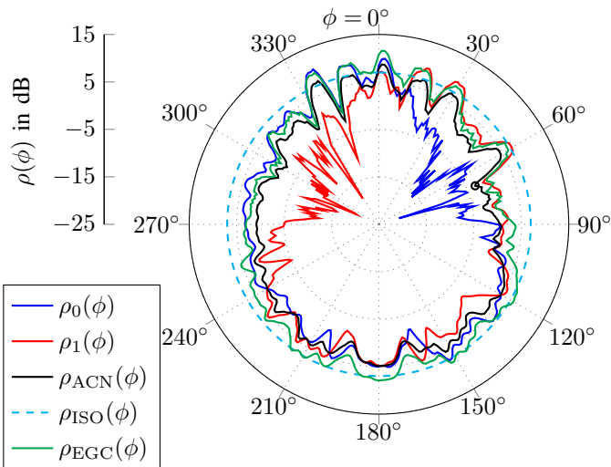
Fig. 3. \rho(\phi) of the two monopoles mounted on the roof of a vehicle and the ACN. The monopoles exhibit nonisotropic power gains. P_T/P_n = 1 and K = 5 .
