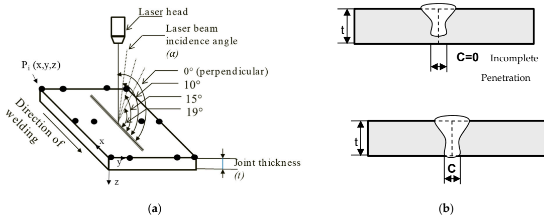
Figure 2. Case study parameters: (a) laser beam incident angle, joint thickness, and 12 points to measure distortion ( X:[0,75,150] ; Y:[0,5,35,40] ; Z:[0] ); (b) laser weld bead geometry showing incomplete joint penetration (in which C = 0 ) and complete joint penetration.
