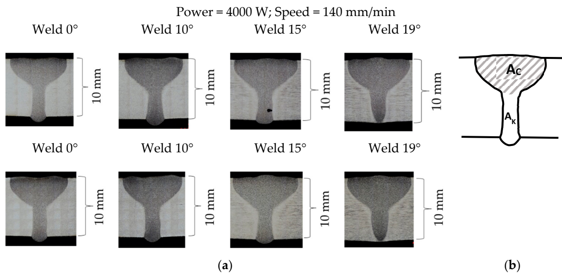
Figure 6. (a) Cross sections of the four BOP-welds. Each cross section has been replicated twice. (b) Generic representation of a laser weld bead, which can be divided in two main areas: conduction area ( A_C ) and keyhole area ( A_K ).
