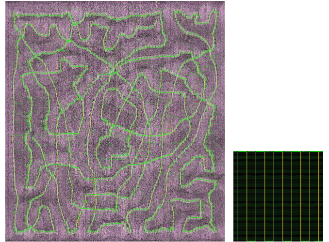
Fig. 4. 8640-channel cell-based and full-custom 28-nm autocorrelator layouts (relative scaling shown).
