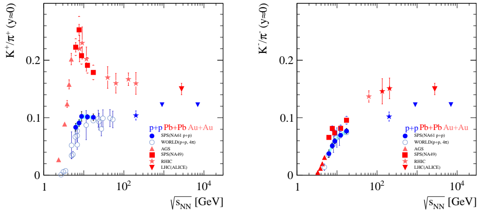
Figure 5: Left: the energy dependence of the K^+/\pi^+ ratio in p+p interactions changes rapidly at the energy where the 'horn' structure is visible in Pb+Pb. Such a behaviour was not predicted in p+p interactions by models, including the Statistical Model of the Early Stage, which predicted the 'horn' structure as a signature of the Quark-Gluon Plasma (QGP). Right: the energy dependence of the K^-/\pi^- ratio in p+p and heavy-ion interactions. The energy dependence of the K^-/\pi^- ratio does not reveal the horn structure since it is not representative of total strangeness production. The world data plotted in both panels is taken from the Ref. [10, 15, 16, 17, 18].
