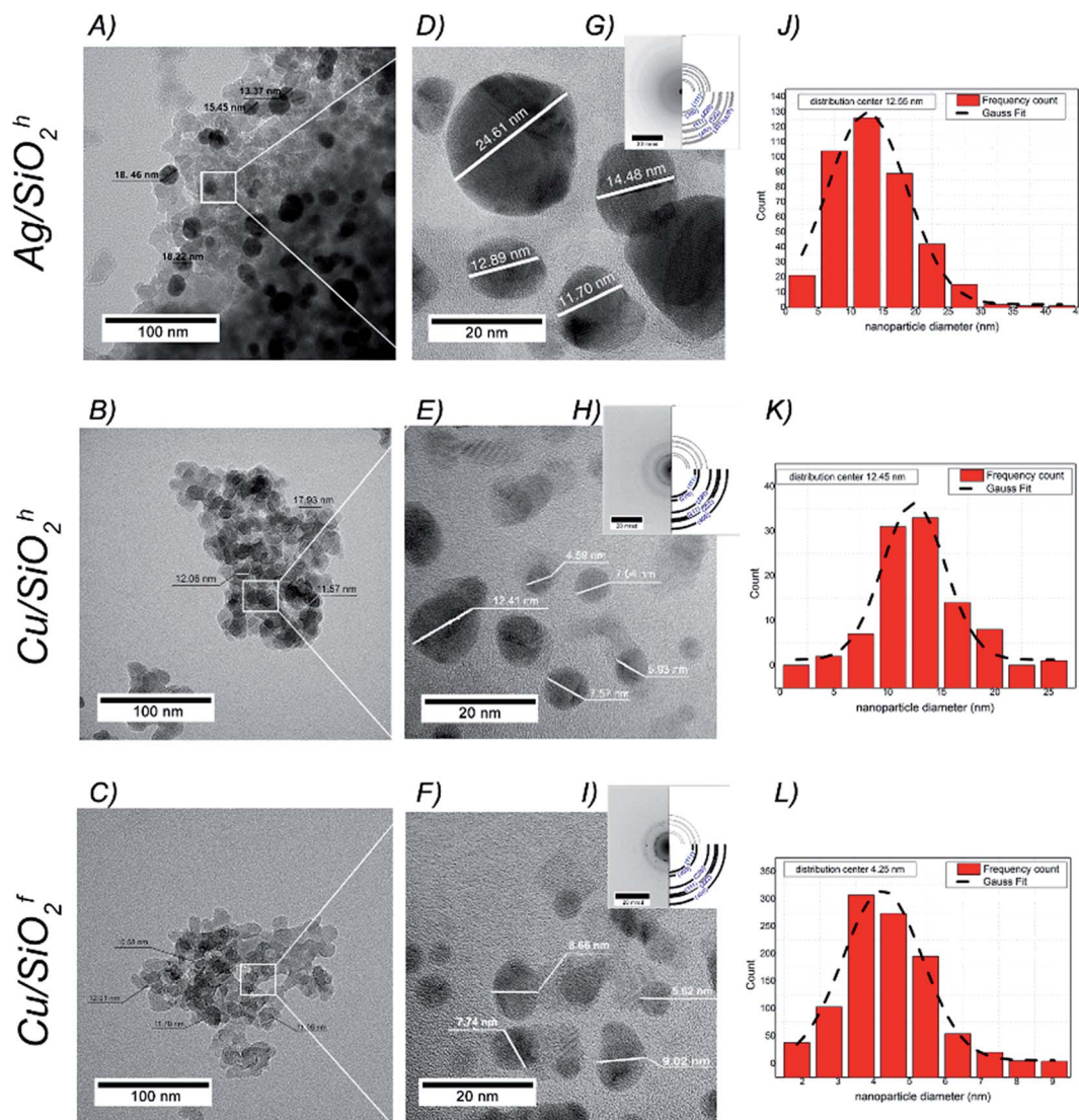
Fig. 3 (A)–(C) TEM micrographs with the scale bar of 100 nm and (D)–(F) with the scale bar of 20 nm obtained for \text{Ag}/\text{SiO}_2^{\text{h}} , \text{Cu}/\text{SiO}_2^{\text{h}} and \text{Cu}/\text{SiO}_2^{\text{f}} nanocomposites. The brightest objects mean silica matrix, whereas the dark ones are silver or copper particles embedded into the silica matrix. (G)–(I) Insets show SAED patterns for each nanocomposite (left site) with theoretical fitting (right site) while (J)–(L) the particle size distribution for each system was based on three different TEM images.
