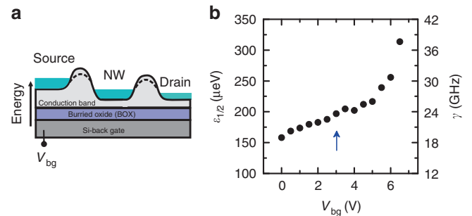
Fig. 4 Low temperature limit. a Schematic of the conduction band edge along the nanowire channel. The quantum dot-reservoir tunnel barriers can be controlled “in-situ”. b The full width at half maximum \epsilon_{1/2} and the tunnel rate \gamma as a function of back-gate voltage V_{bg} . The arrow indicates the V_{bg} at which thermometry was performed. The error bars are smaller than the size of the dots. The error includes the uncertainties in the gate lever arm \alpha and the \epsilon_{1/2} measurements
