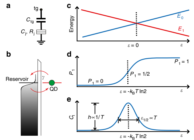
Fig. 1 Theory. a Circuit equivalent of the quantum dot (QD)-reservoir system. b Schematic of cyclic electron exchange between a discrete energy level of a QD and a thermally broadened electron reservoir. c Energy diagram of a fast driven two-level-system (TLS) with discrete energies E_0 and E_1 , across a charge degeneracy point. d Probability P_1 of an electron to be in the QD as a function of energy level detuning \varepsilon . e Tunneling capacitance C_t as a function of \varepsilon
