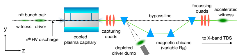
Figure 8. Schematic of the proposed beamline scheme for separation of driver and witness bunches in high-power multi-bunch trains.
