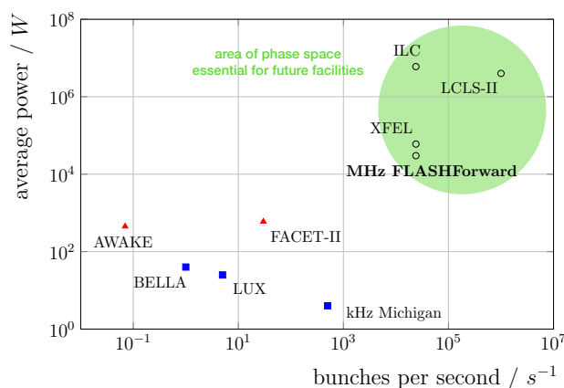
Figure 6. Average-power capabilities (as a function of the number of bunches per second their drivers can deliver) of state-of-the-art LWFA (blue squares) and PWFA (red triangles) facilities. The white circles represent the state-of-the-art or next generation of photon science and collider facilities. By implementing certain infrastructural changes to FLASHForward, PWFA research would move into the region of phase space necessary for future facilities.
