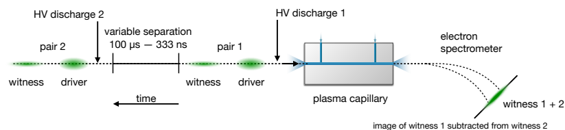
Figure 7. Schematic of the proof-of-principle effective MHz experimental setup illustrating two driver-witness bunch-pairs with variable separation interacting with two distinct plasmas generated by consecutive high-voltage discharges.
