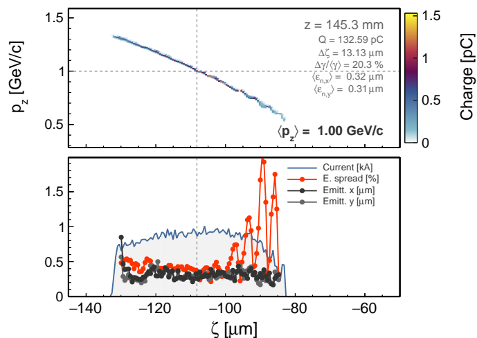
Figure 3. (Top) Longitudinal phase-space and (bottom) slice energy spread (red), normalised transverse emittance (black, grey), and peak current (blue) of the witness bunch after a propagation distance of \sim 15 cm simulated in OSIRIS 3D [20–22]. A typical FLASHForward 1 GeV drive beam with 0.1% relative energy spread, \sigma_z = 25 \mu\text{m} rms length, \sigma_{x,y} = 6 \mu\text{m} rms width, 2 \mu\text{m} normalised transverse emittance, a charge of 500 pC, and a peak current of 2.4 kA was chosen to drive the wake. The plasma electron density at the peak of the ramp was 4 \times 10^{17} \text{cm}^{-3} (ten times higher than that of the flat-top) with a downramp length of \sim 100 \mu\text{m} .
