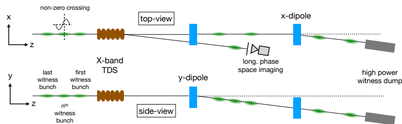
Figure 9. Schematic of the proposed beamline modifications necessary to utilise the FLASHForward X-TDS for characterisation of MHz PWEA bunch trains.
