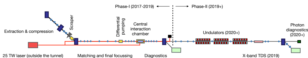
Figure 2. Schematic of the FLASHForward experimental beamline, highlighting major sections and components.
