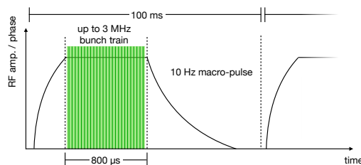
Figure 5. Schematic of the 10 Hz macro-pulse and MHz bunch train structure available to FLASHForward for high-power experimentation.
