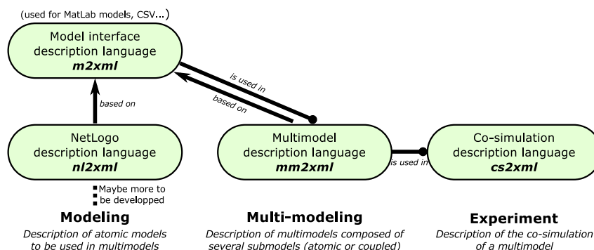
Figure 2: Scheme of MECASYCO DSL.
