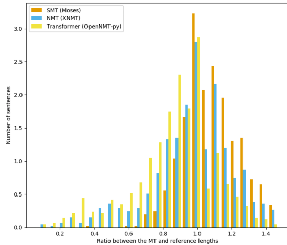
Figure 2: Distribution of Cr#pbank translations length ratio w.r.t ground truth translations.
