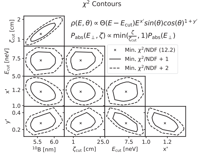
FIG. 6. Contours of \chi^2 in the parameter space of l_{^{10}\text{B}} , \zeta_{\text{cut}} , E_{\text{cut}} , x' , and y' . On each subplot, the projection of the five-dimensional \chi^2 contours and the global minimum is shown.
