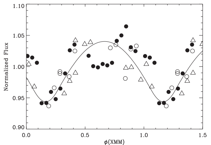
Figure 10. Normalized XMM-Newton and STIS data aligned. Filled circles are for the XMM-Newton fluxes, open circles for the N IV data, and open triangles for the Si IV data. The STIS data have been shifted to align them with the XMM-Newton data to emphasize how they all appear to follow a single period.
