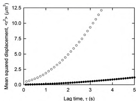
Figure 4. Mean-squared displacement (MSD) of a Janus particle in 5% \text{H}_2\text{O}_2 in the absence (open circles) and presence (black filled circles) of 20 nm nanoparticles. The MSD of a Janus particle in the absence of 20 nm particles depended on the square of lag time, while the MSD depended linearly on lag time following the addition of the nanoparticles. The \tau^2 dependence indicated propulsion (see eq 8), while the \tau indicated a purely Brownian motion (see eq 9).
