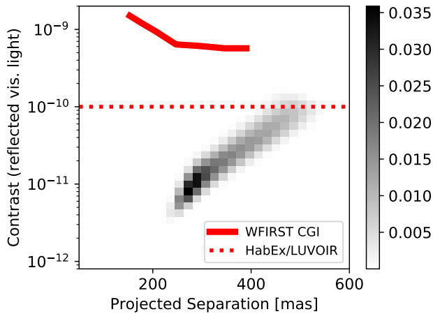
Figure 9. Two-dimensional histogram showing the posterior in planet contrast/projected separation, approximating the planet as a Lambertian disk with an albedo of 0.5. This plot shows a “snapshot” of the posterior in time on 01-01-2025. Darker grey indicates higher probability. The predicted post-processing detectability floor for the WFIRST CGI b in narrow FOV mode is shown as a red solid line, where regions above the line are detectable. The dotted line shows the HabEx/LUVOIR performance requirement. HR 5183 b is likely not detectable in reflected light with the WFIRST CGI or HabEx/LUVOIR.
