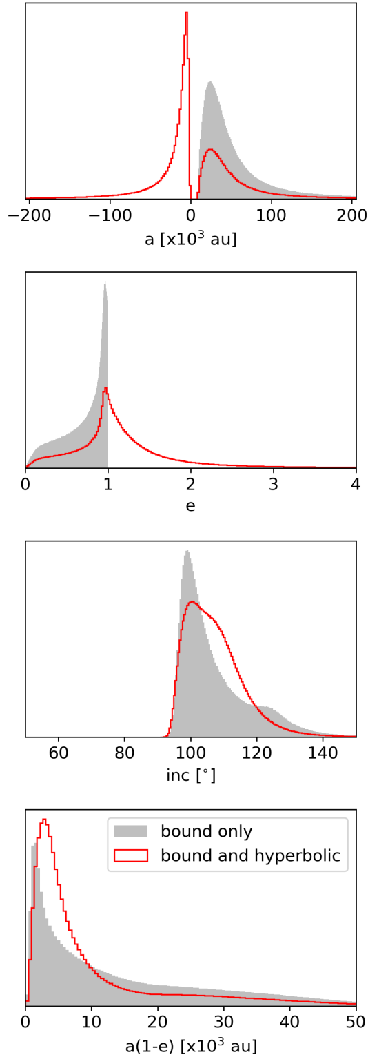
Figure 7. Bound (grey solid) and all (red line) solutions for the orbit of HIP 67291 and HR 5183. These are normalized, so even though the grey PDF is a subset of the red PDF, the grey exceeds the red in places. These solutions may not be accurate if there are undetected massive companions around HIP 67291. High eccentricities and edge-on orbits are preferred. Although small values of a(1-e) (neglecting unbound hyperbolic orbits) are possible, the most probable value occurs at 1,000 au, and the median at 10,000 au, too widely separated to affect the planet HR 5183 b. The most probable orbital period is almost 1 Myr.
