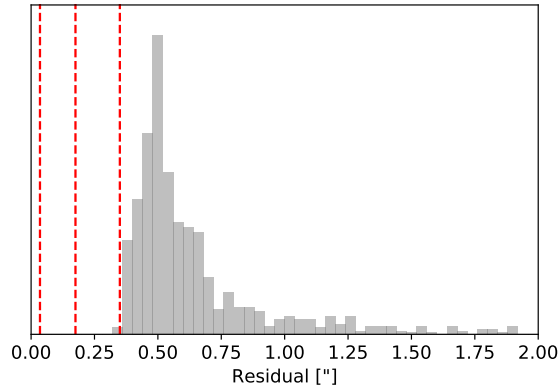
Figure 12. Histogram of the residual values of simulated Gaia astrometric orbits to straight-line fits. To be detectable, the residual must be greater than five times the Gaia measurement uncertainty on the position of HR 5183. Red vertical dotted lines are shown at 1, 5, and 10- \sigma . See Section 6 for a complete description of this algorithm. Based on this analysis, 100% of simulated orbits of HR 5183 b are 5- \sigma detectable with Gaia.
