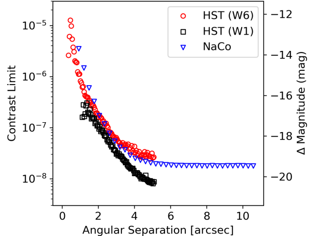
Figure 5. 1\text{-}\sigma point-source detection limits for HR 5183 computed with NaCo on the VLT in the Ks-band, and with HST-STIS using WedgeA-0.6 (W6) and WedgeA-1.0 (W1). See Appendix B for details. We did not detect companions to HR 5183 in these images.
