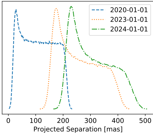
Figure 8. Posterior distributions of the projected separation ( \rho ) of HR 5183 b from its primary at three future epochs. The time of periastron passage is precisely constrained to be 01-2018 from the RVs, and accordingly, the separation posterior generally increases over the next 5 years. In 2024, HR 5183 b will be separated from its host by more than 200 mas with 95% confidence.
