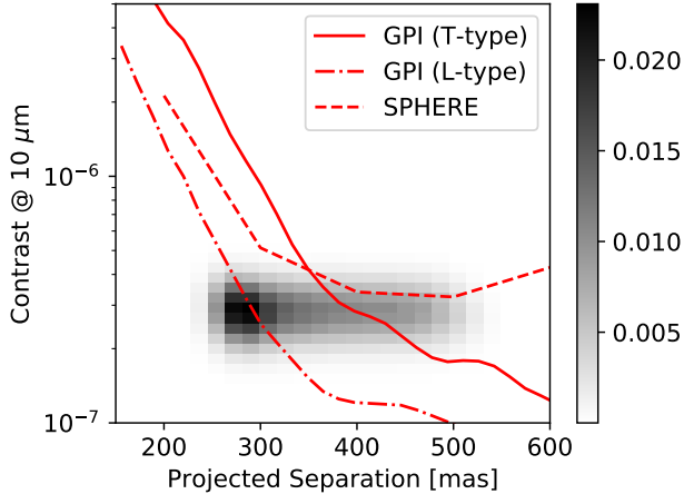
Figure 10. Same as Figure 9, except contrast is calculated in the thermal infrared, assuming T_{\text{eff}} is the equilibrium temperature at periastron. The red lines show the post-processing detectability floors of the Gemini Planet Imager (GPI) and SPHERE, infrared imagers currently in operation (though importantly without 10\mu\text{m} capabilities). These predictions indicate that HR 5183 b could be imageable with a 10\mu\text{m} infrared imager in the next 5 years, bearing in mind the important caveat that the thermal background is higher at 10\mu\text{m} than at GPI/SPHERE observation wavelengths, potentially negatively impacting contrast capabilities.
