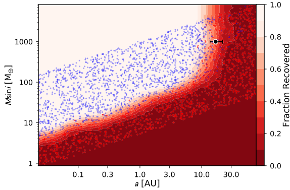
Figure 4. Sensitivity of the HR 5183 RV time series to injected planetary signals as a function of semimajor axis ( a ) and minimum mass ( M \sin i ). Each point corresponds to an injected radial velocity signal. Blue dots were detected, while red dots were not. The solid-color background shows the fraction of signals that were recovered, corresponding to the probability of detection. The parameters of HR 5183 b are shown as a black point with error bars (the uncertainty on M \sin i is too small see). Our data are sensitive to less massive, shorter-period planets out to the orbit of HR 5183 b.
