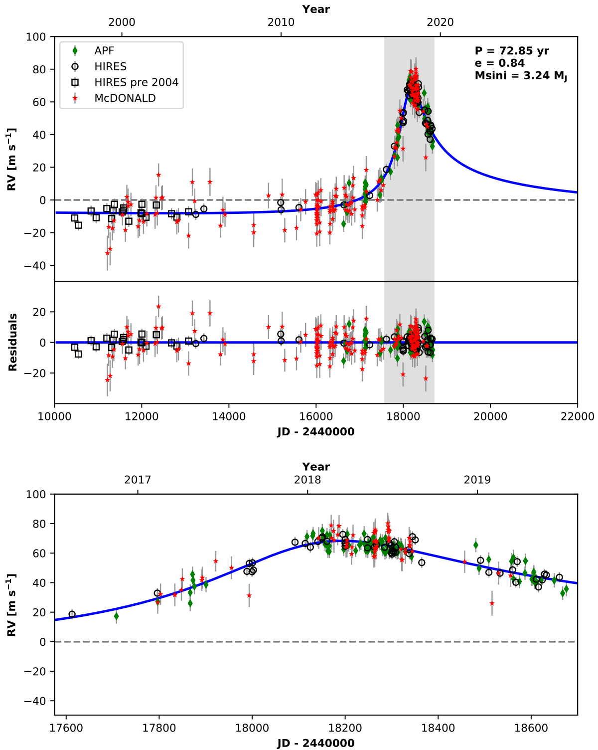
Figure 1. Top: RVs of HR 5183 from the Keck-HIRES, McDonald-Tull, and APF-Levy spectrographs as a function of time. Error bars show observational errors and instrument-specific jitter values added in quadrature. The best-fit Keplerian orbit is shown (blue solid line). Residuals are inset below. Bottom: close-up of the grey region in top plot. The RV curve peaks in January 2018 during periastron passage, and declines monotonically afterward in all three data sets.
