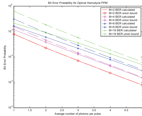
Fig 1. BER for optical homodyne detection.
