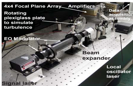
Fig. 3. Coherent combining experiment at the Jet Propulsion Laboratory, NASA.
