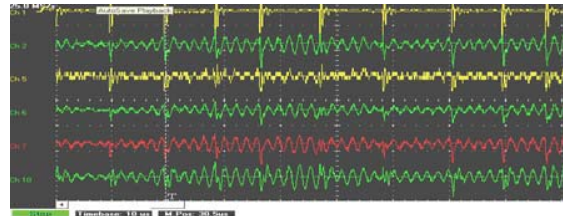
Fig. 4. PPM Beatnotes plus lower frequency oscillation observed using the GaGe Scope data acquisition assembly.
