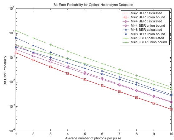
Fig. 2. BER for optical heterodyne detection.
