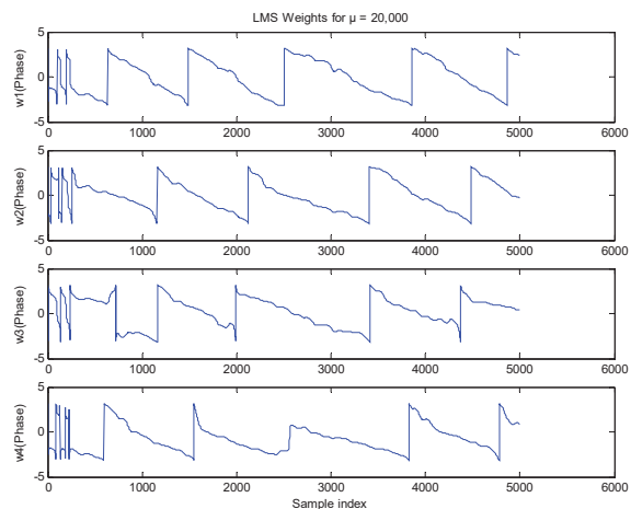
Fig. 12. Phase of the weights with \mu=20,000 .
