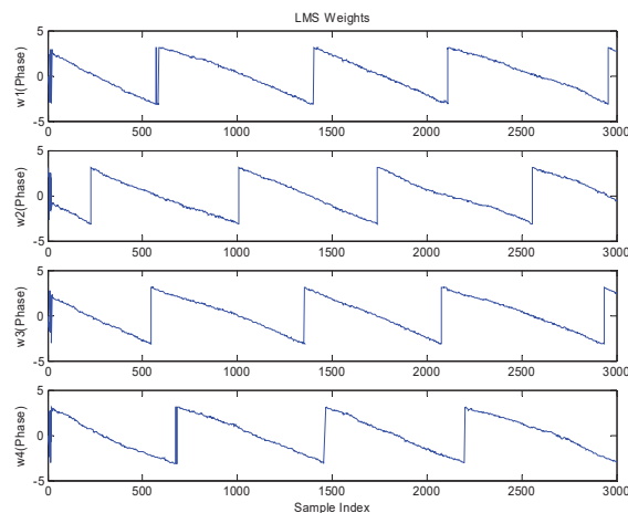
Fig. 8. Phase of the weights for \mu=1000 .
