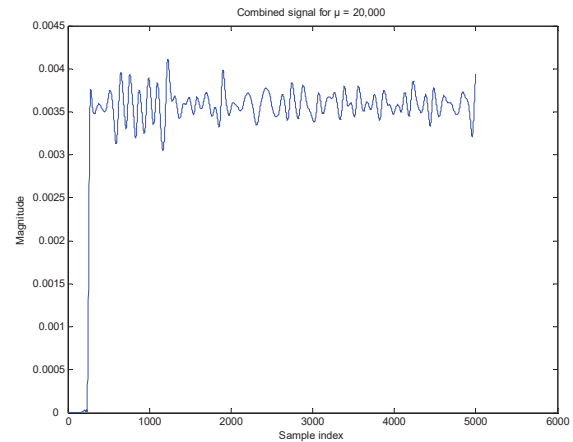
Fig. 11. Combined output power of the beatnote signal in the presence of simulated atmospheric turbulence with \mu=20,000 .
