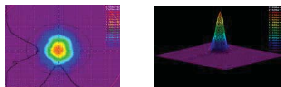
Fig. 6. Beam profile of the signal laser with ideal conditions (no atmospheric turbulence).
