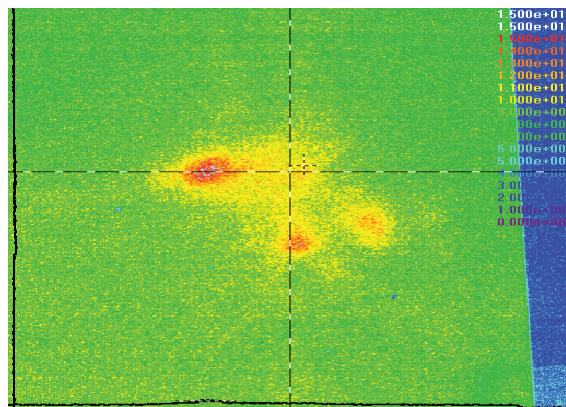
Fig.10. Intensity distribution of the signal laser in the presence of simulated atmospheric turbulence conditions.
