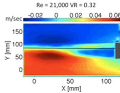
Figure 12. V_{\text{mean}} of high Re Top Row: Re = 21,400 VR = 1.00 Middle Row: Re = 22,100 VR = 0.55 Last Row: Re = 21,000 VR = 0.32
