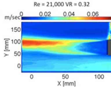
Figure 16. V_{\text{prime}} RMS of high Re.
