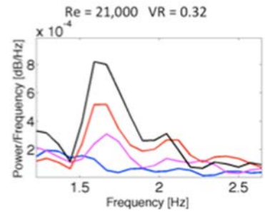
Figure 20. PSD of high Re. Top Row: Re = 21,400 VR = 1.00 Middle Row: Re=22,100 VR=0.55 Last Row: Re=21,000 VR=0.32
