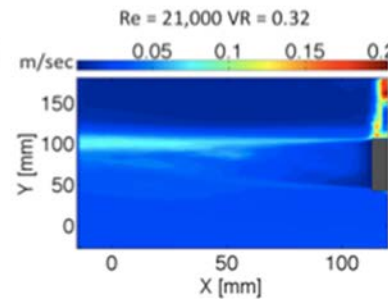
Figure 9. U_prime RMS of high Re.
