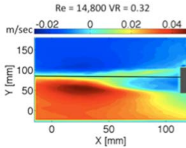
Figure 11. V_{\text{mean}} of med Re. Top Row: Re = 15,200 VR = 0.98 Middle Row: Re = 15,700 VR = 0.57 Last Row: Re = 14,800 VR = 0.32
