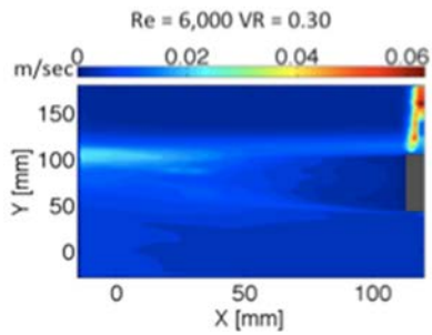
Figure 7. U_prime RMS of low Re.
