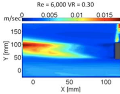
Figure 13. V_{\text{prime}} RMS of low Re.
