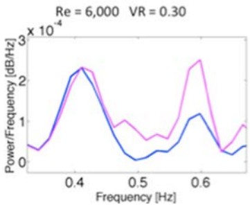
Figure 18. PSD of low Re. Top Row: Re = 6,200 VR = 0.93 Middle Row: Re=6,000 VR=0.46 Last Row: Re=6,000 VR=0.30
