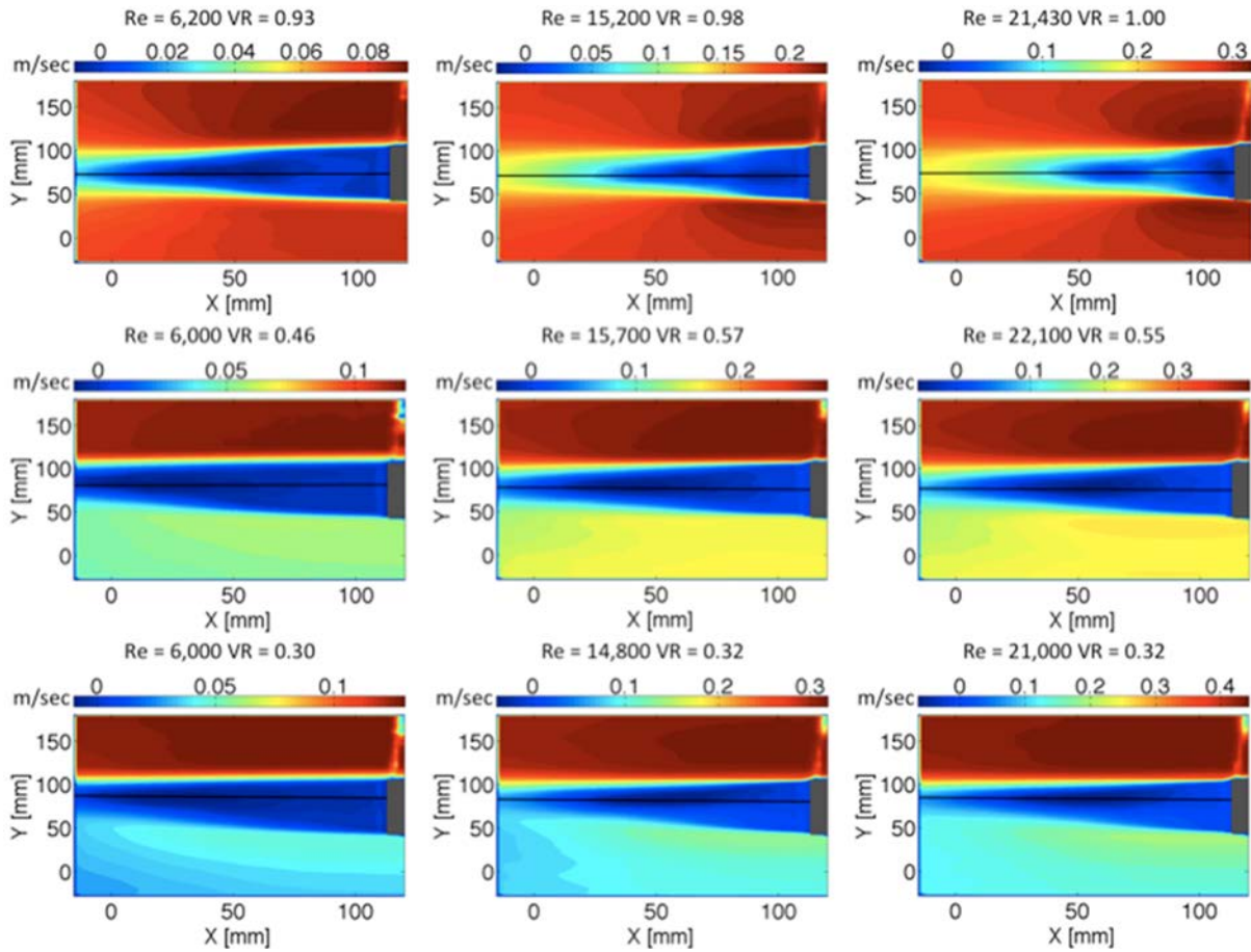
Figure 4. U_{\text{mean}} of low Re.
