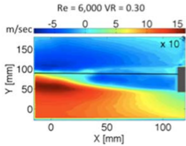
Figure 10. V_{\text{mean}} of low Re. Top Row: Re = 6,200 VR = 0.93 Middle Row: Re = 6,000 VR = 0.46 Last Row: Re = 6,000 VR = 0.30
