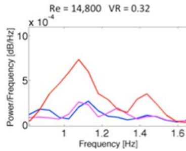
Figure 19. PSD of med Re. Top Row: Re = 15,200 VR = 0.98 Middle Row: Re=15,700 VR=0.57 Last Row: Re=14,800 VR=0.32
