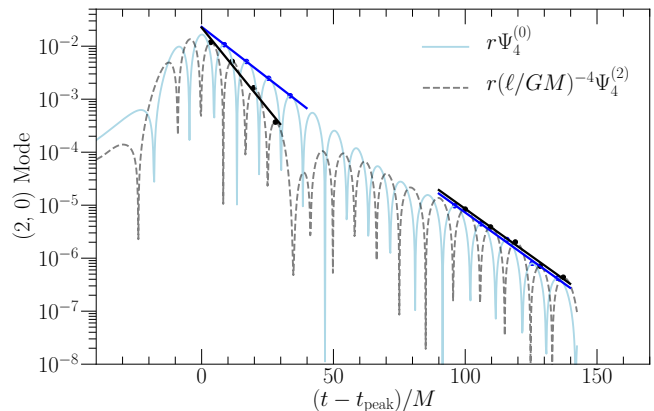
FIG. 13. The real parts of r\Psi_4^{(2)} and r\Psi_4^{(0)} for \chi = 0.1\hat{x} . We fit a line (on this semi-log plot) to the peaks of the gravitational waveform during various stages of the post-merger waveform (black for r\Psi_4^{(2)} , blue for r\Psi_4^{(0)} ). Early on in the waveform, r\Psi_4^{(2)} and r\Psi_4^{(0)} have different damping times, whereas later in the waveform, they have the same damping time. This suggests that at late times, r\Psi_4^{(2)} is well-modeled as a QNM on a pure Kerr background.
