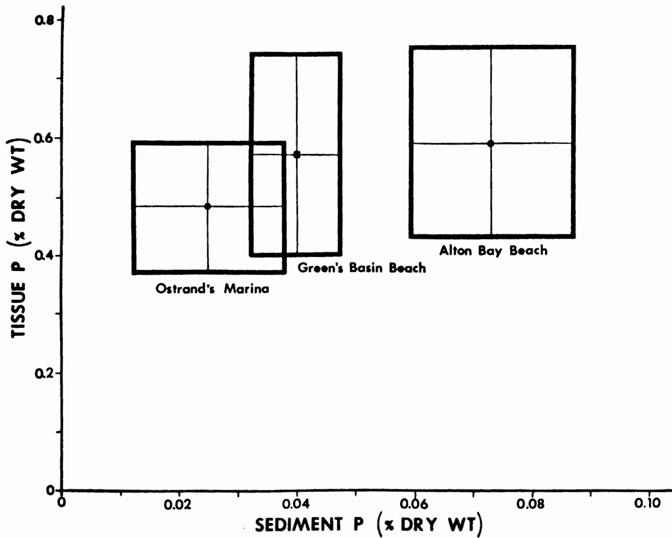
Figure 13. Mean tissue phosphorus as related to mean sediment phosphorus at three study sites, summer 1975. ( \pm one standard deviation)
