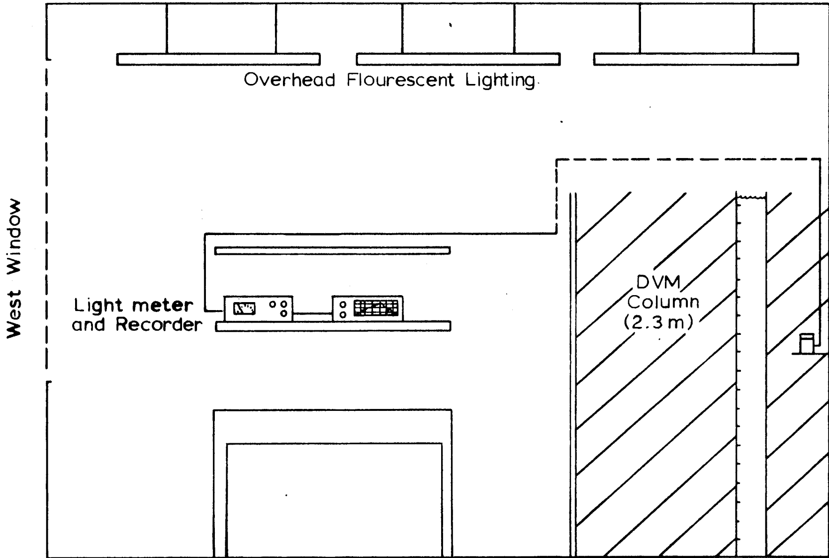
Figure 1. DVM Room illustration arrangement of columns and lighting.
