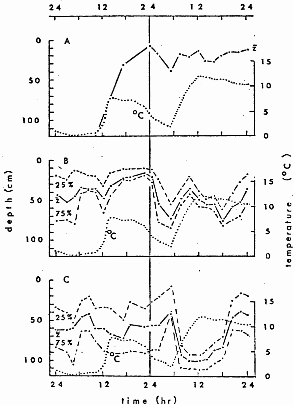
Figure 29. Column studies at Toolik, Alaska. \bar{z} = mean depth; 25%, 75% = quartiles; ^{\circ}\text{C} = temperature. A: Bosmina longirostris , adults, 29 VI 76. B: Daphnia middendorffiana , juveniles, 28-29 VI 76; C: Daphnia longiremis cephela, adults, 28-29 VI 76. See table 6 for correlation coefficients of light and mean depth, and temperature and mean depth.
