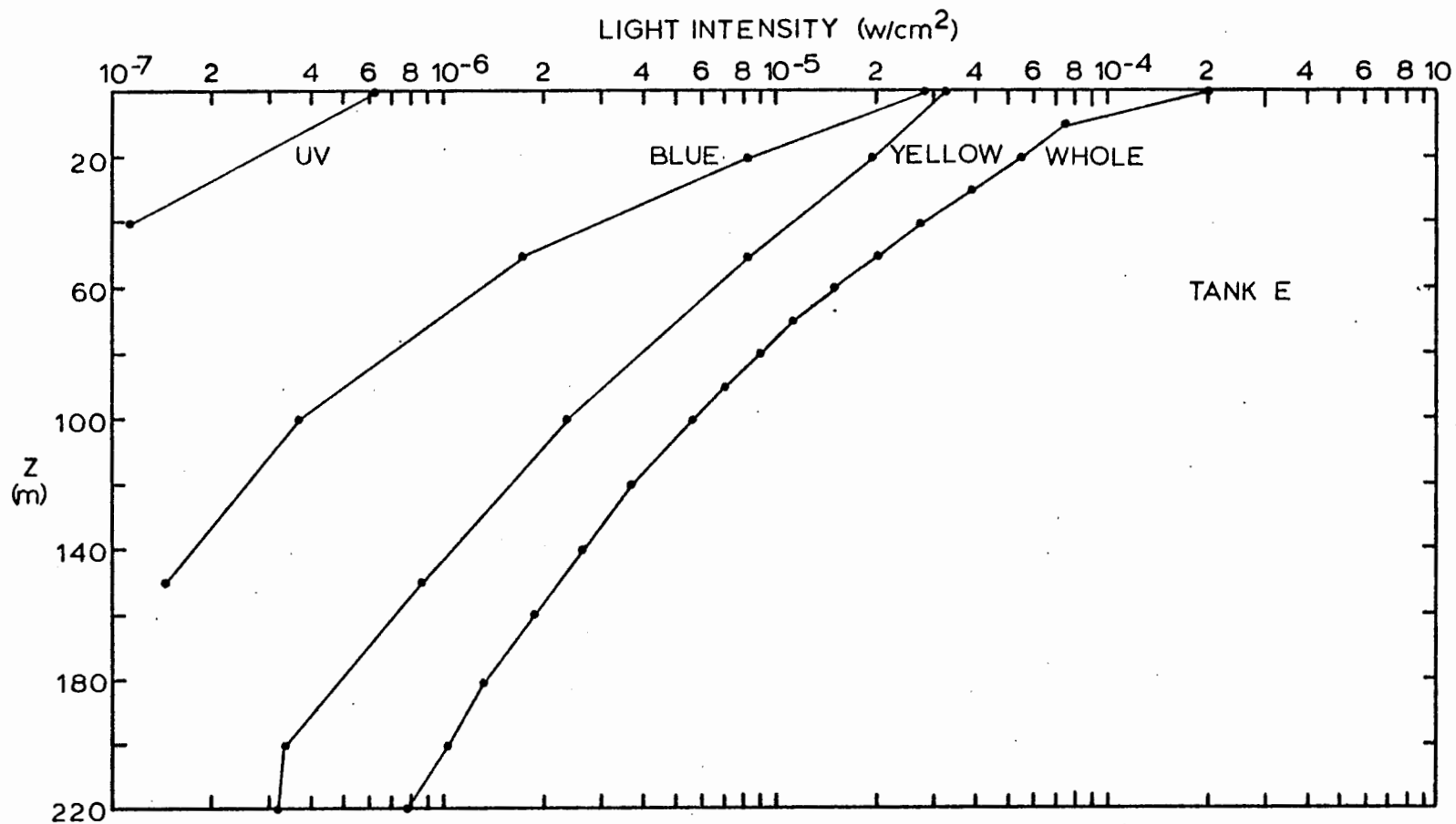
Figure 10. Light transmission of various wavelengths in DVM Room, Column E. See Fig. 6 for additional details.
