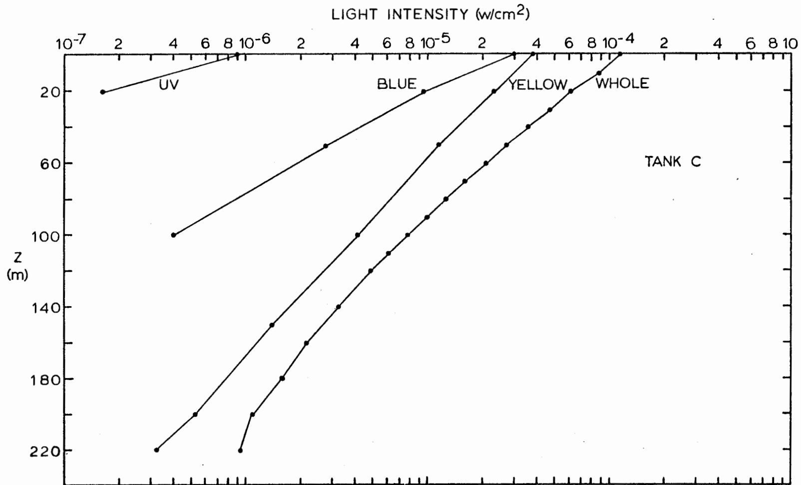
Figure 8. Light transmission of various wavelengths in DVM Room, Column C. See Fig. 6 for additional details.
