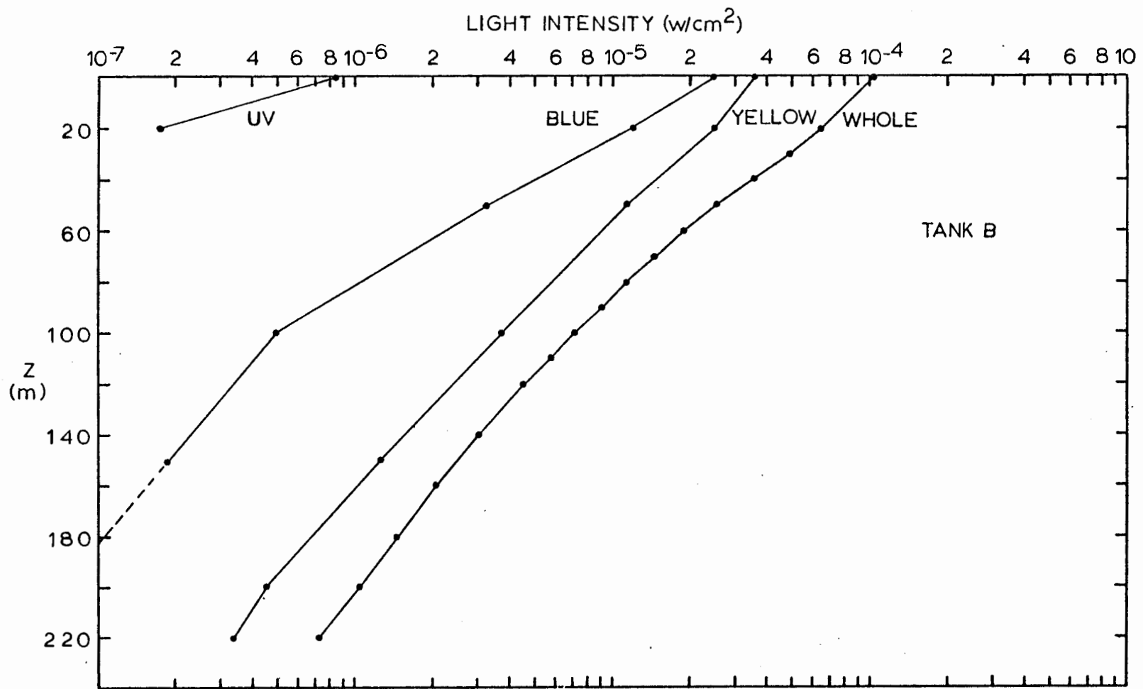
Figure 7. Light transmission of various wavelengths in DVM Room, Column B. See Fig. 6 for additional details.
