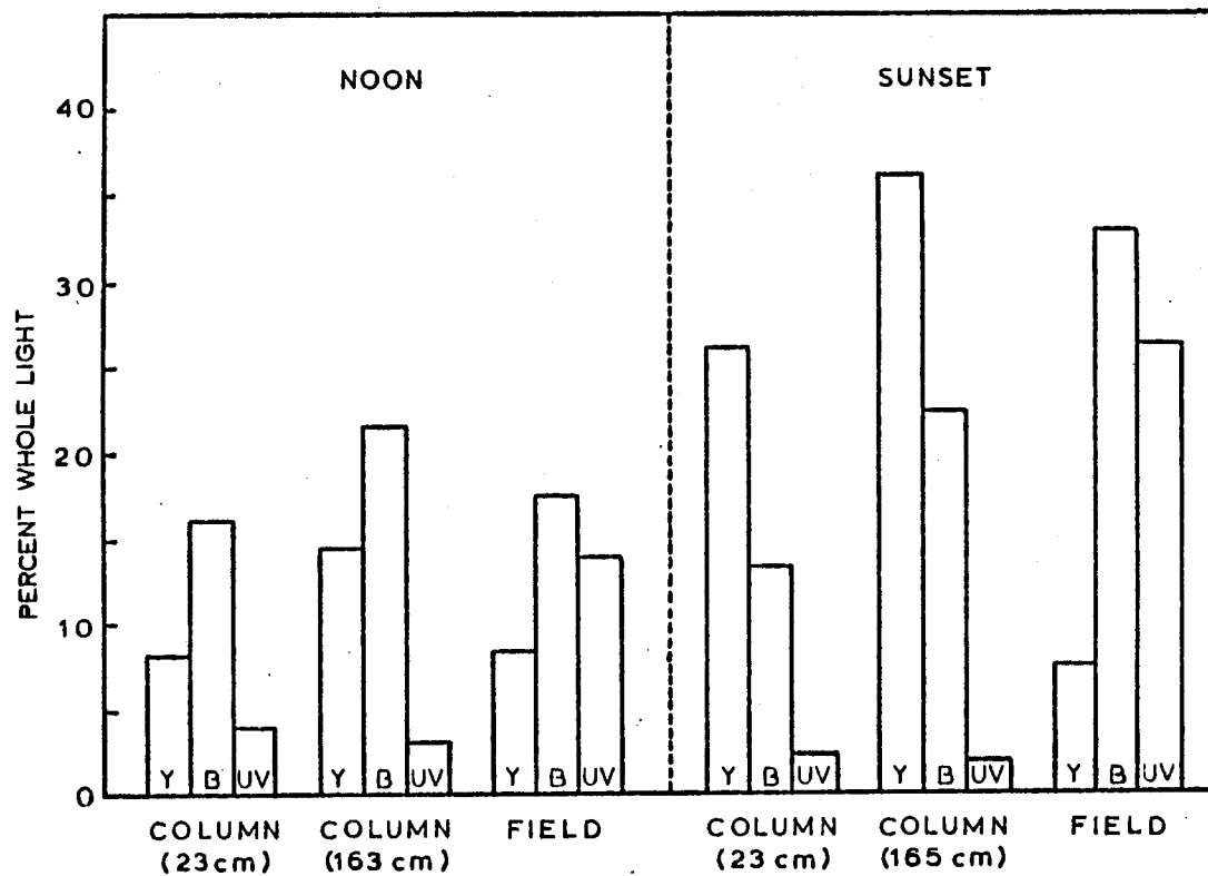
Figure 5. Spectral distribution of light in the DVM Room and outside under natural light expressed as the percentage of light measured without a filter (whole light). Peak transmittance of narrow band filters: ultraviolet (365 nm), blue (428 nm) and yellow (569 nm). Measurements taken within a 15-min. period at noon (1245-1300 h) and sunset (1814-1833 h) on 12 April, 1976.
