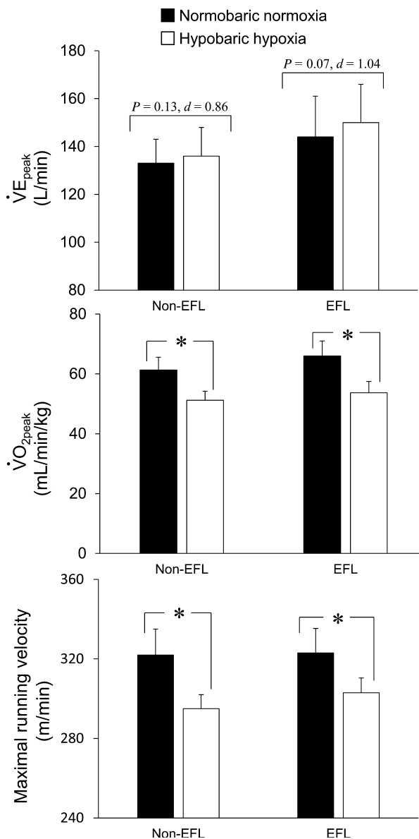
Figure 3. Peak ventilation ( \dot{V}E_{\text{peak}} ), peak oxygen uptake ( \dot{V}O_{2\text{peak}} ), and maximal running velocity under normobaric normoxic and hypobaric hypoxic conditions. Non-EFL, runners without expiratory flow limitation; EFL, runners with expiratory flow limitation. * P < 0.05 hypobaric hypoxia versus normobaric normoxia.
