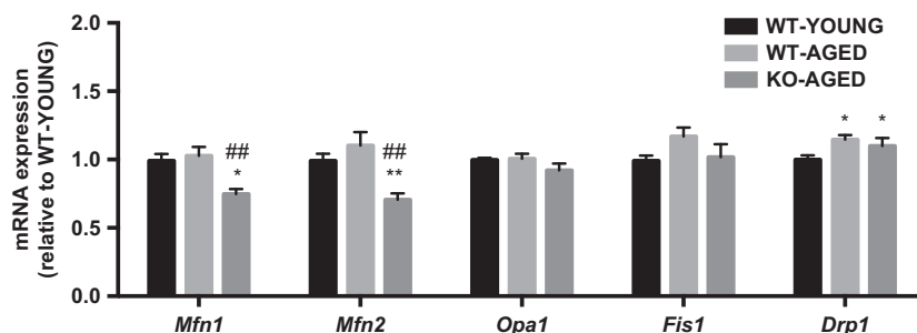
Figure 6. Mitochondrial dynamics genes in aged Nrf2 KO mice. Data are presented as mean \pm SEM n = 5-7 in each group. *P < 0.05 , significant difference versus WT-YOUNG. ^{##}P < 0.01 , difference versus WT-AGED. WT, wild type; KO, knockout.
