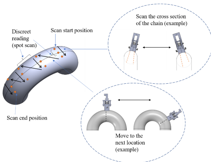
FIGURE 11. Proposed mooring chain scanning steps (for an automated manipulator)
