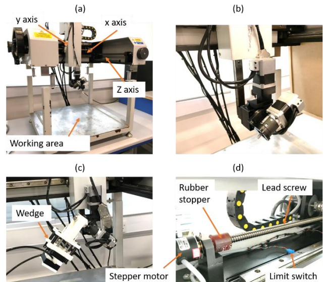
FIGURE 16. Automated 5DOF manipulator. (a) 5axis manipulator test rig. (b) 2 rotary axis closer view. (c) Wedge attachment. (d) axis components
