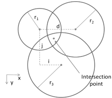
FIGURE 4. Calculation of the intersection point of three spheres array directions
