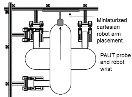
FIGURE 22. Proposed miniaturized robotic manipulator attachment.
