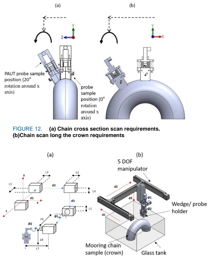
FIGURE 13. (a) schematics of the proposed manipulator. (b) CAD model of the proposed manipulator.
