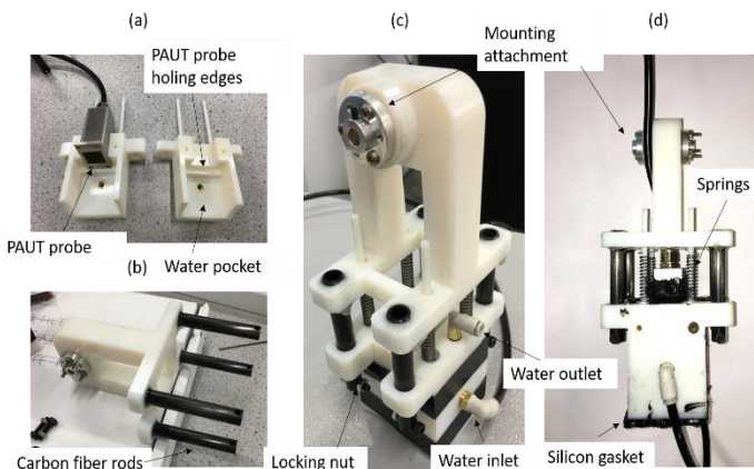
FIGURE 15. Prototype of the continuous water supply wedge. (a) Water pocket and the PAUT probe. (b) Manipulator attachment. (c) &(d)
