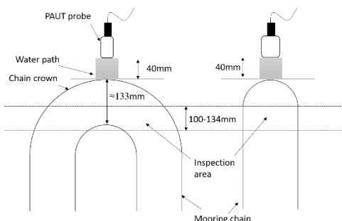
FIGURE 9. NDT probe holder/ wedge design requirements.
