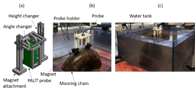
FIGURE 5. (a) CAD model of the Probe holder. (b) experimental setup. (c) Full experimental setup; submerged condition
