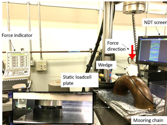
FIGURE 14. Spring force requirement test rig
