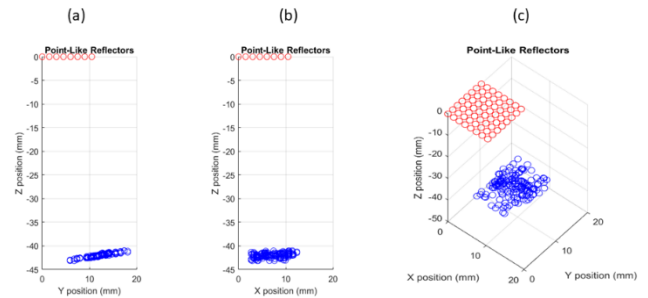
FIGURE 8. Example surface mapping results for the point like reflectors projection algorithm (a) y-z mapping. (b) x-z mapping. (c) x-y-z surface mapping sample.
