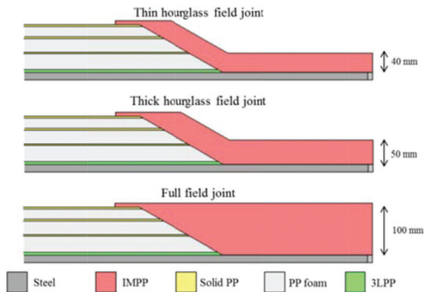
Figure 7. Modelling of field joints in COMSOL.
