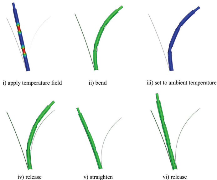
Figure 13. Bend cycle steps modelled in Abaqus.
