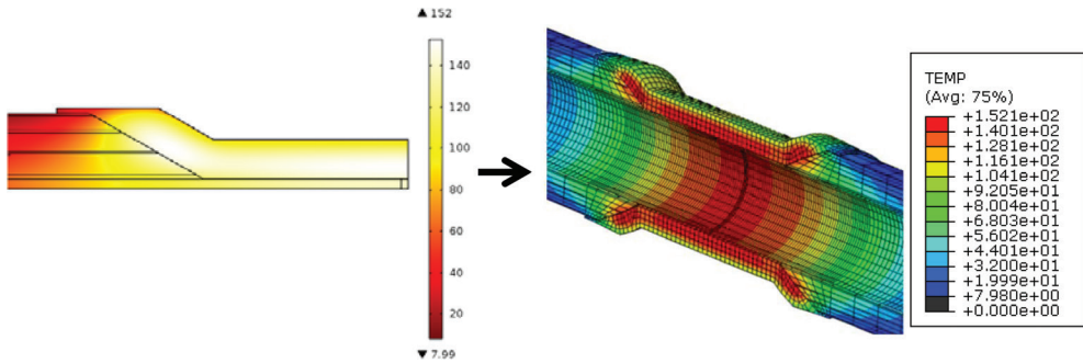
Figure 12. Example of transferral of COMSOL temperature output to a discrete field in Abaqus.
