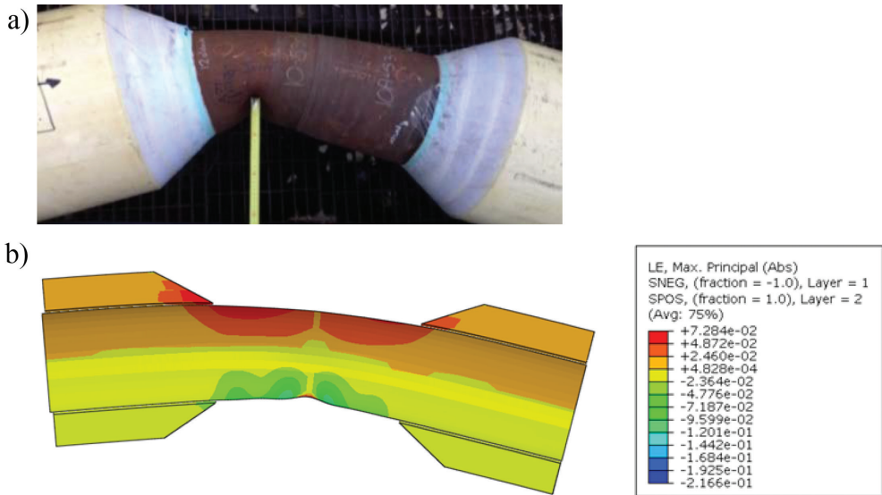
Figure 14. Bending of field joint with no coating; (a) experimental observation and (b) numerical prediction of strain field.
