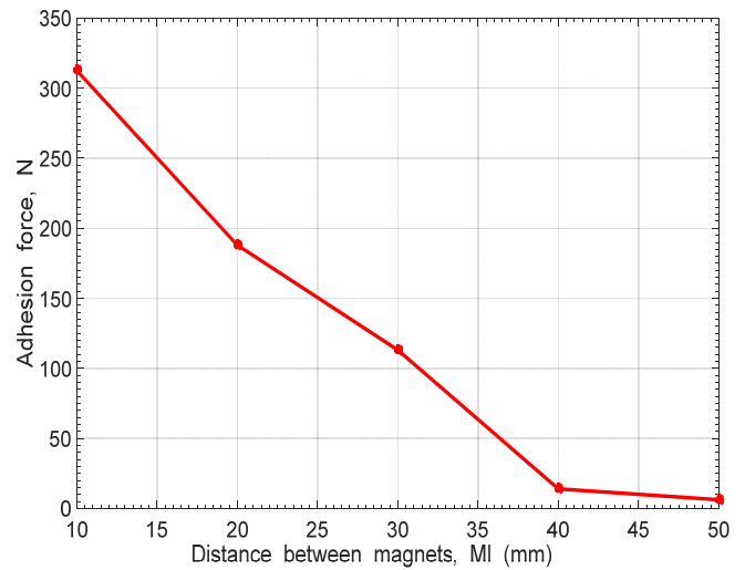
Fig. 12 Measured adhesion force [18]
