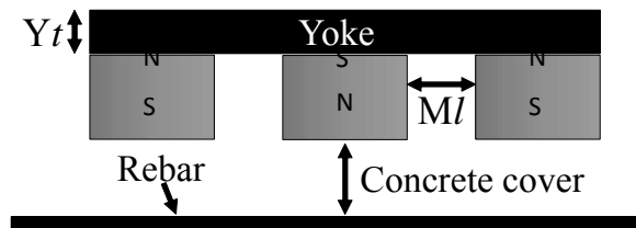
Fig. 8 Proposed structure of the adhesion module
