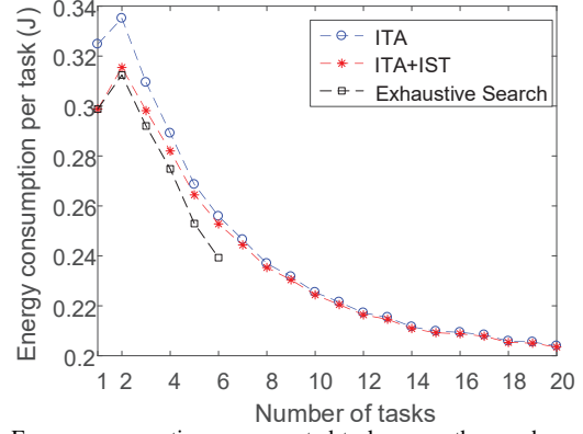
Fig. 3. Energy consumption per executed task versus the number of tasks in D2D-assisted MEC networks.
