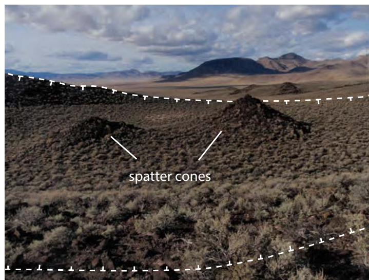
Figure 20. Two spatter cones on the floor of a larger crater (rim shown with dashed line). The largest spatter cone is ~5 m high. Location: 38°31'43"N, 115°57'06"W.
