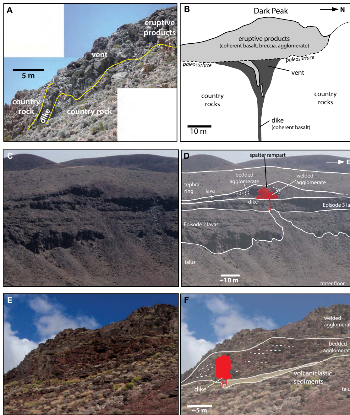
Figure 18. Examples of exposed dike vent (conduit) transitions. (A) Oblique photo of east-facing side of Dark Peak, a scoria cone remnant (episode 1) showing upper few meters of feeder dike, upward flaring to fill a vent structure, and eruptive products. (B) Simplified sketch of the Dark Peak dike, vent fill, and eruptive products. Both A and B are based upon Harp and Valentine (2015), and are located at 38°06'51"N, 116°10'30"W. (C) Part of the northern crater wall of Lunar Crater maar, which exposed cross section of an episode 4 spatter rampart. (D) Photograph showing thin (~50 cm) subvertical dike that can be traced to ~15 m below the base of the spatter rampart. The dike widens to ~1 m within the upper 2 m of the paleosurface (the top of episode 3 lava), and extends upward and merges with a domain of densely welded agglomerate that grades laterally to bedded, progressively less welded agglomerate, and a lava flow of the same material. Location: 38°23'14"N, 116°03'56"W. (E) Oblique view of an episode 2 scoria cone remnant in the Reveille Range, which was fed by a 30–50-cm-wide, en echelon dike. (F) Photograph showing the dike, which flares to ~4 m width where it intrudes poorly to moderately welded, bedded agglomerate of the cone. Location: 38°04'16"N, 116°08'03"W.
