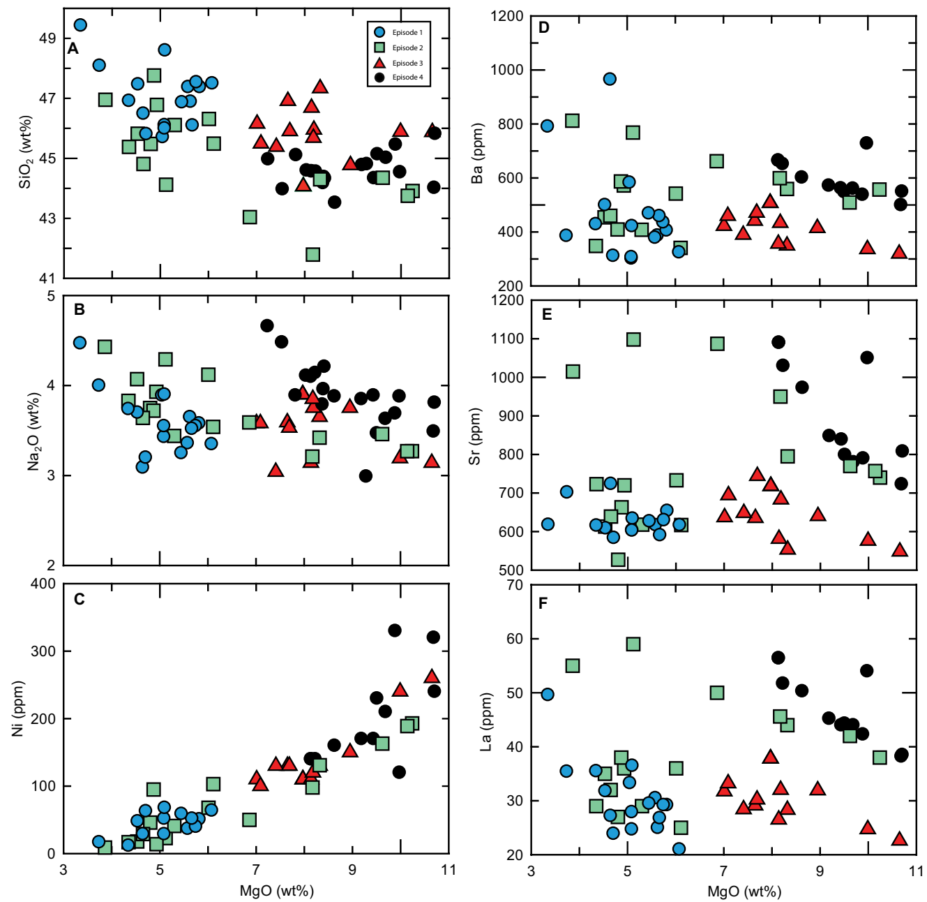
Figure 9. Abundances of SiO 2 , Na 2 O, and selected trace elements plotted against MgO for all four basaltic episodes at Lunar Crater volcanic field.
