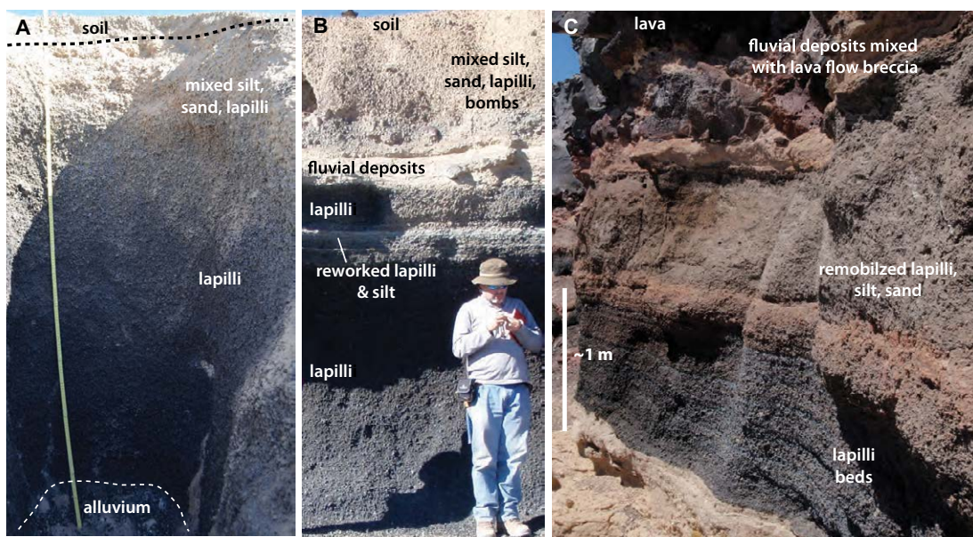
Figure 26. Example tephra fall deposits in the Lunar Crater volcanic field. (A) Southern lobe of ca. 35 ka Marcath tephra at a location 2.3 km south of the main cone (38°27'58"N, 115°58'41"W). Deposit consists of a single massive scoria lapilli bed on alluvium. It is capped by an eolian desert soil. The upper portion of the deposit contains silt and fine sand that has infiltrated from above, and the deposit is locally bioturbated (burrows). Vertical stick is 190 cm long. (B) Tephra quarry ~1 km north of the northern end of Easy Chair ramparts, along Highway 6. Lower portion is a single massive bed of well-sorted scoria lapilli, overlain by bedded silt and scoria interpreted to be reworked material, and overlain by an ~30-cm-thick massive scoria lapilli bed. Material labeled fluvial deposits is bedded and cross-bedded fine sand, silt, and lapilli, with scour and fill structures locally cutting into the underlying scoria lapilli bed. Uppermost mixed silt, sand, lapilli, and bombs are material from a nearby (~300 m to peak) eroded scoria cone mixed with eolian sediment. Desert soil (disturbed here by quarrying) with stone pavement caps the sequence. Location: 38°27'57"N, 116°01'12"W. (C) Tephra fall deposit in western Reveille Range. Planar parallel beds of well-sorted scoria lapilli in lower part of exposure are overlain by mixed silt, sand, and lapilli (reworked) and by fluvial deposits containing basalt and Oligocene ignimbrite clasts, all capped by episode 1 lava. Location: 38°01'25"N, 116°13'54"W.
