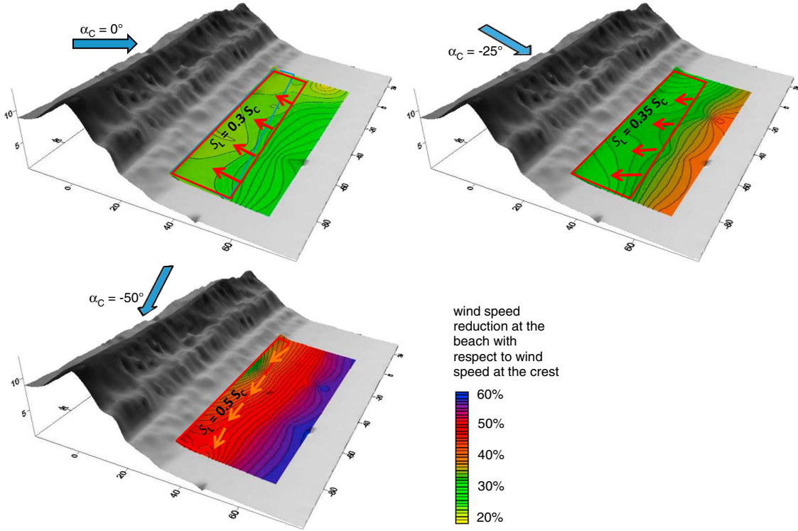
Figure 10. Wind speed reduction at the beach surface with respect to the incoming wind speed for perpendicular ( \alpha_C = 0^\circ ), slightly oblique ( \alpha_C = -25^\circ ), and oblique ( \alpha_C = -50^\circ ) offshore winds. The maps show mean values of S_L/S_C at each of the sensors' locations. Contour lines are every 0.01S_L/S_C (i.e., increases of 1%). S_L/S_C consistently increased away from the crest in all \alpha_C scenarios, but the overall reduction and the range of values were different, with similar wind speeds over the beach surface ( S_L ) during perpendicular winds but wind speeds ranging from 30 to 60% during oblique winds. The red polygons cover an approximate area of beach surface where sediment may be transported back to the dune by reversed airflows (directionality represented by the arrows). Perpendicular offshore winds were associated with the widest area but oblique winds resulted in the strongest speeds at the back beach.
