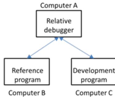
Figure 1: Relative Debugging [2]
