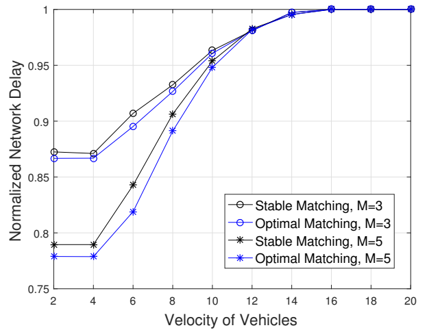
Fig. 7. Normalized delay versus the velocity of vehicles.
