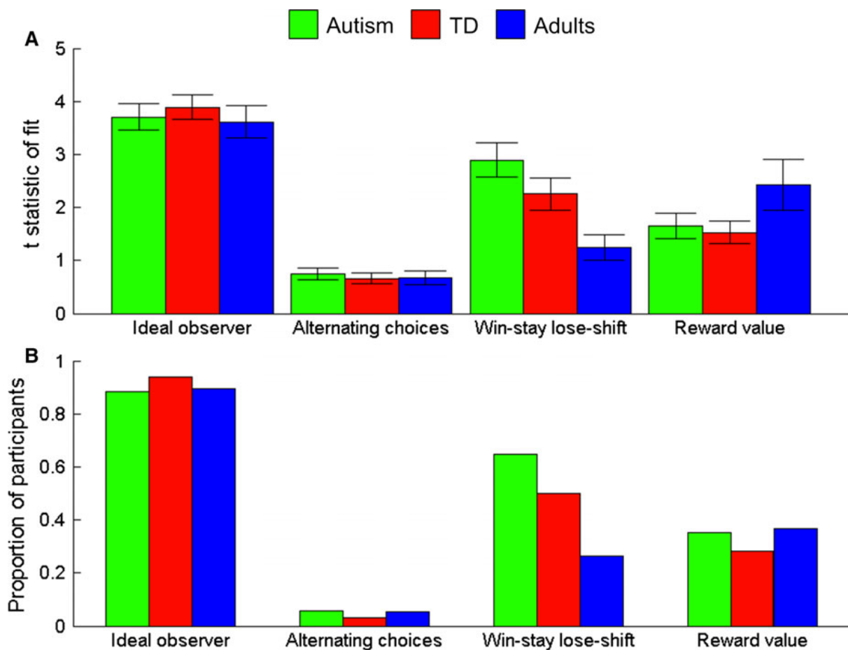
Figure 4. Results of model fitting to participant data
