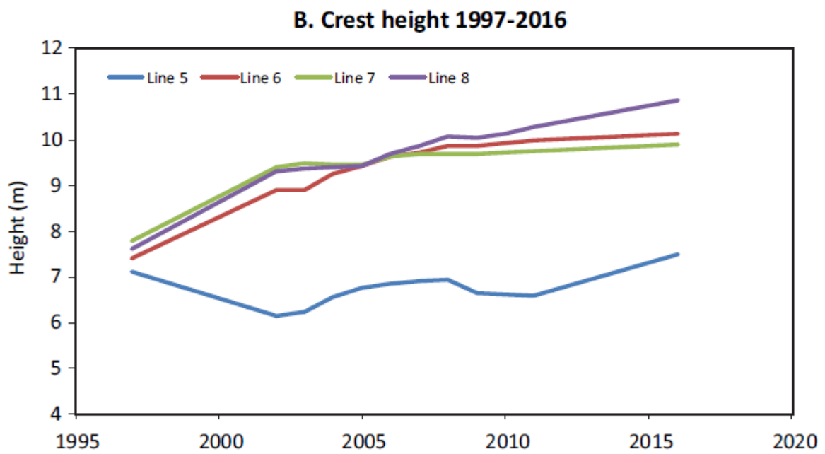
Figure 3: Crest height along lines 5-8 over the period: a) 1953-2016; and b) over the period 1997-2016. Crest elevations are based on DEMs from air photos in 1953, 1971 and 1997, and on survey measurements in the remaining years.
